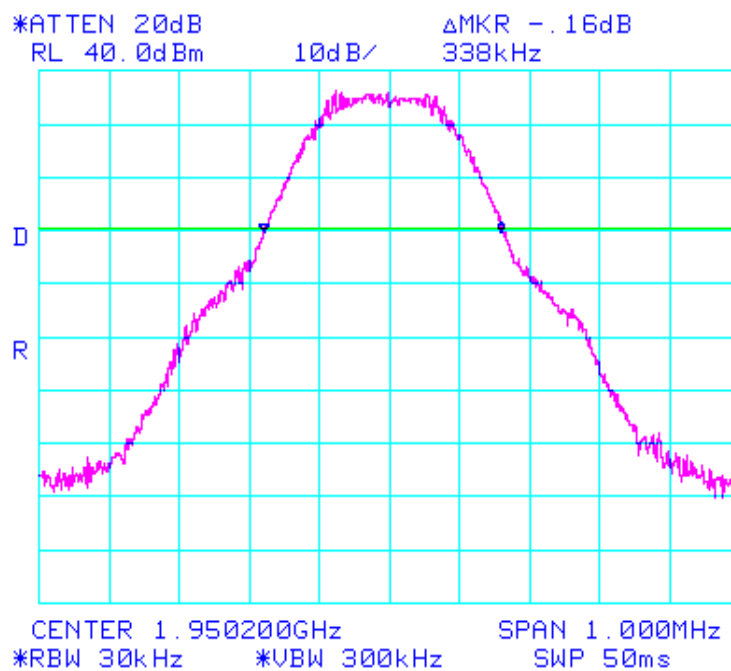
Occupied Bandwidth of the Fundamental signal emi9734
