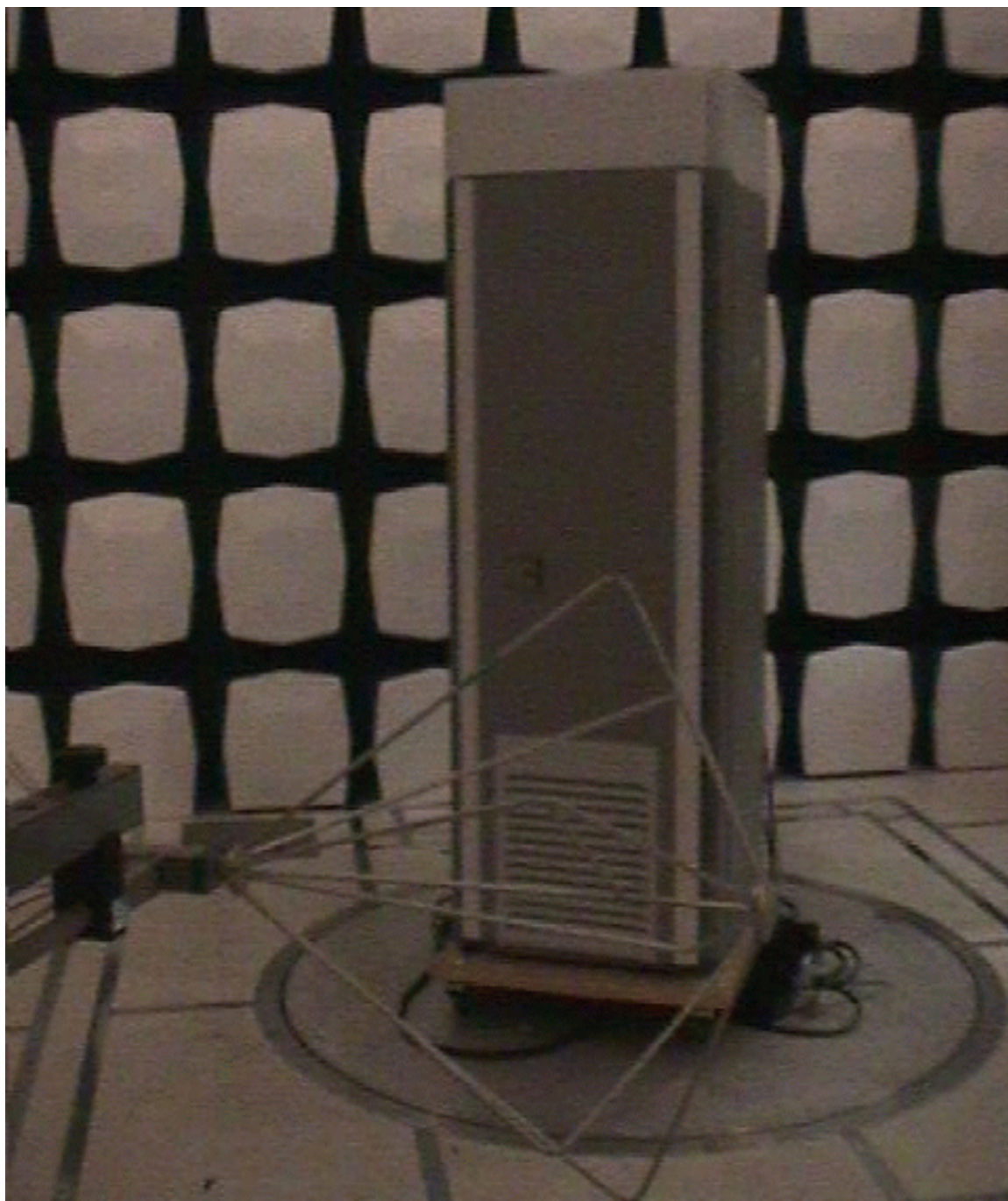
Photograph of Radiated Emissions Test Configuration
