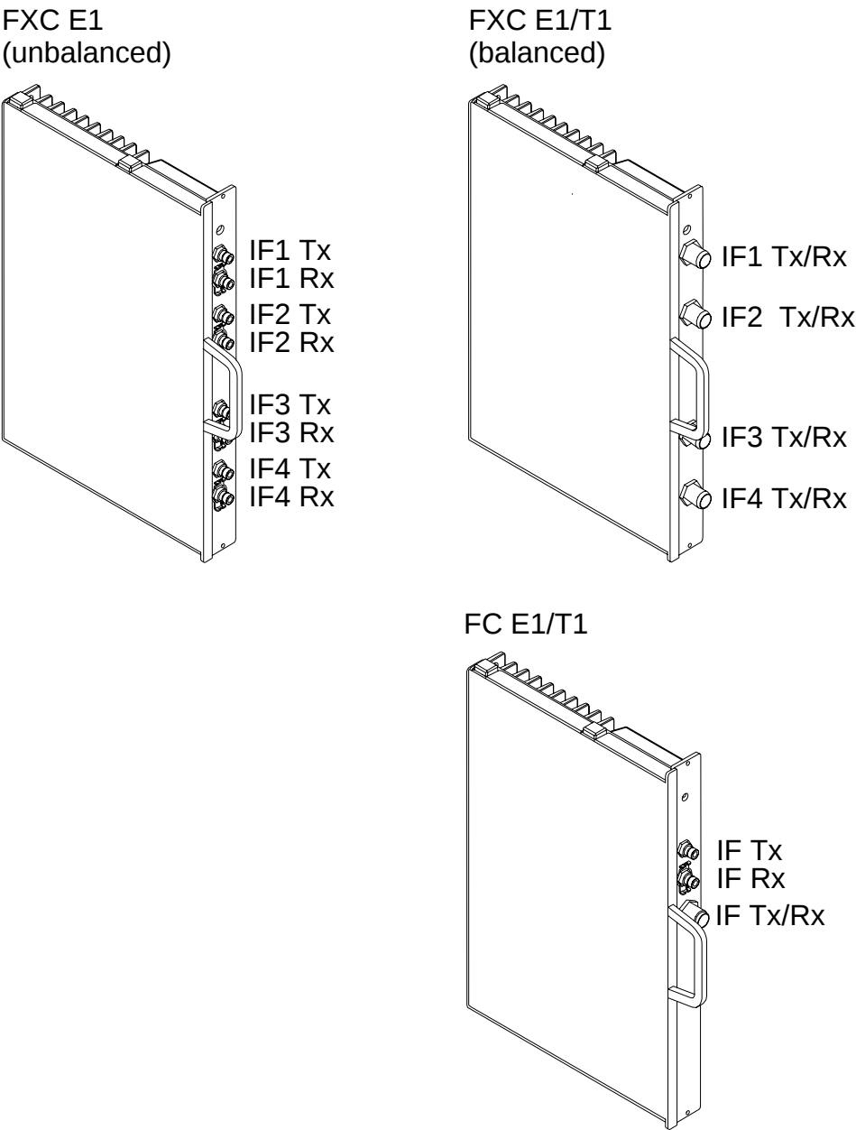
Figure 25. Wireline transmission unit alternatives
