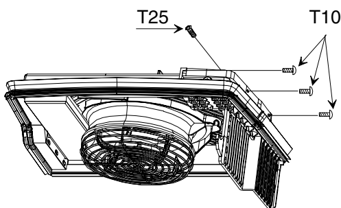
Figure 6. VMFA cooling fan assembly mounting screws
