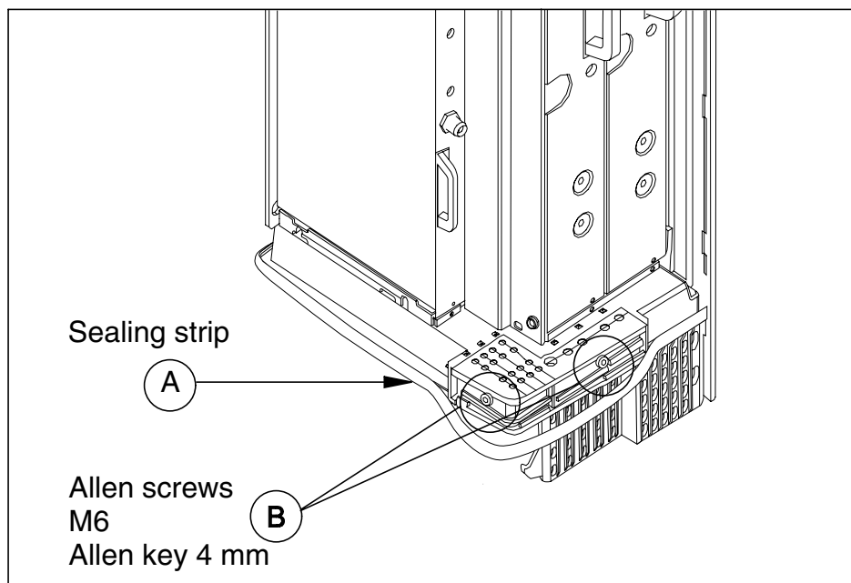
Figure 5. Sealing strip and cable entry block
