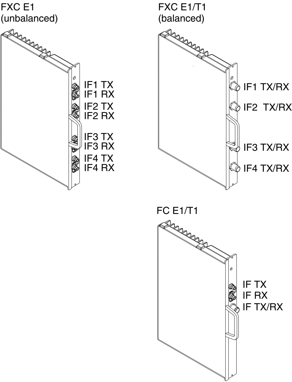
Figure 27. Wireline transmission unit alternatives
