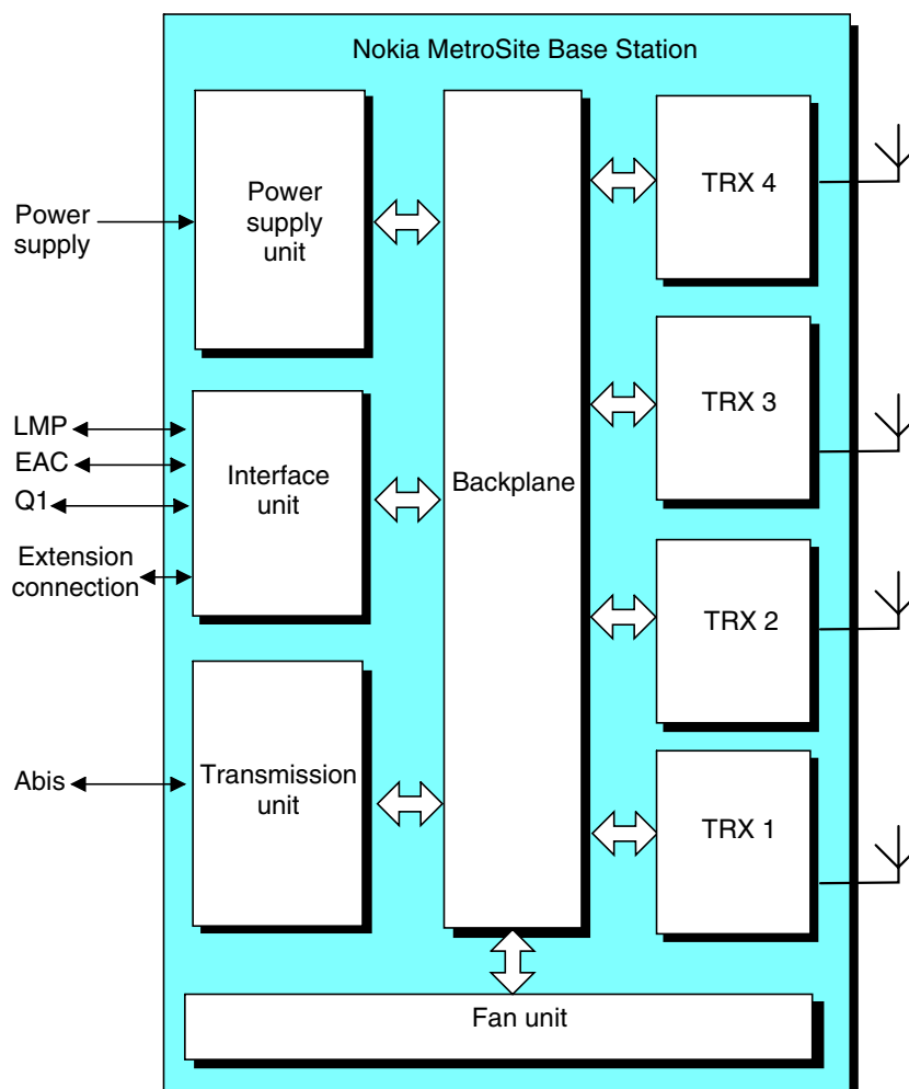
Figure 13. Nokia MetroSite EDGE Base Station block diagram
