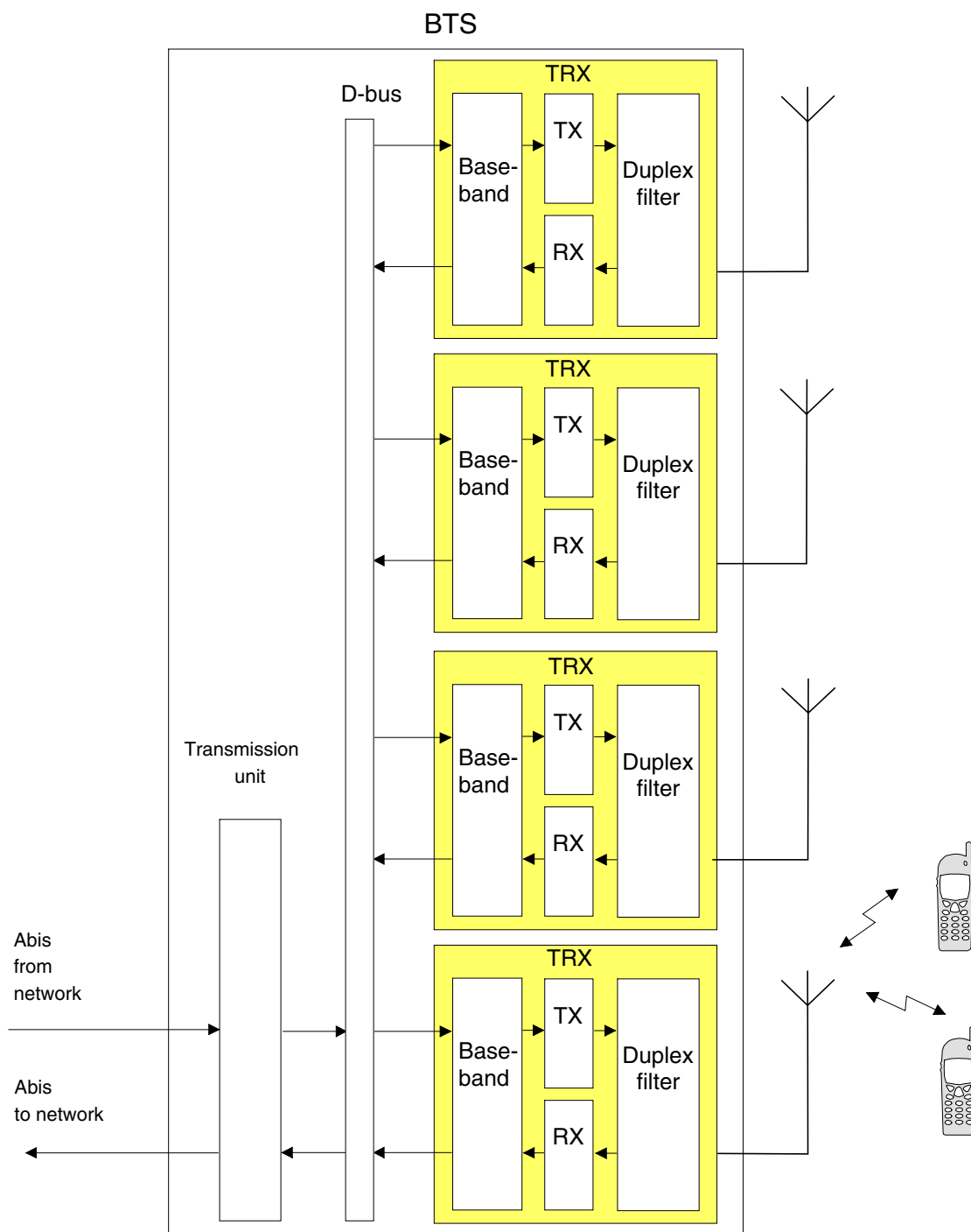
Figure 12. General principle of signalling between network, BTS and mobile station
