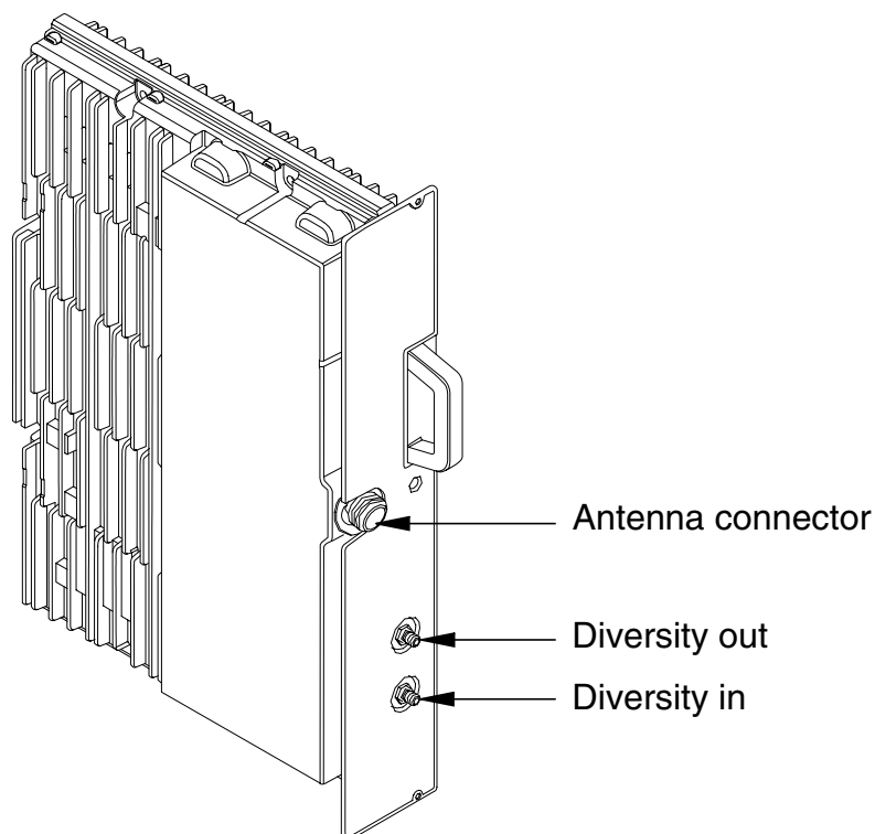
Figure 17. Transceiver unit
