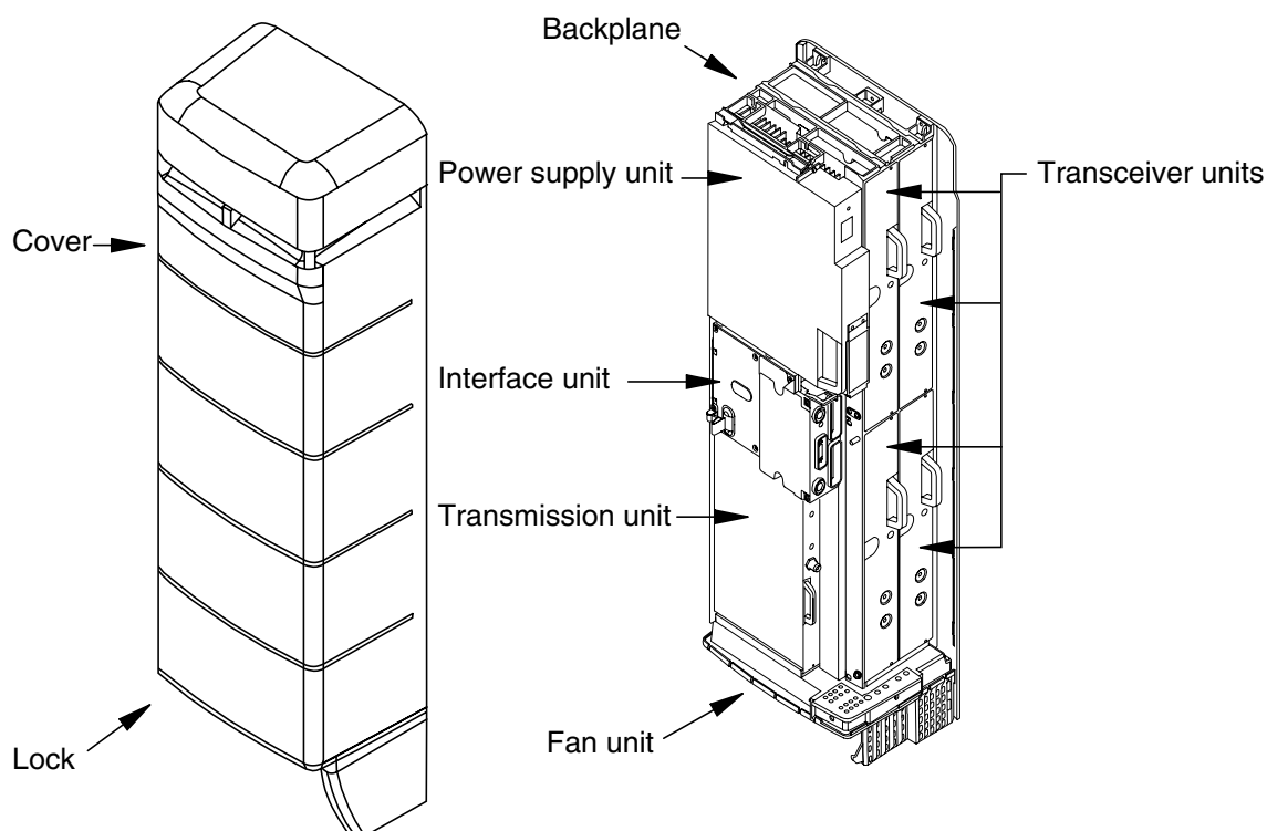
Figure 16. Arrangement of units
