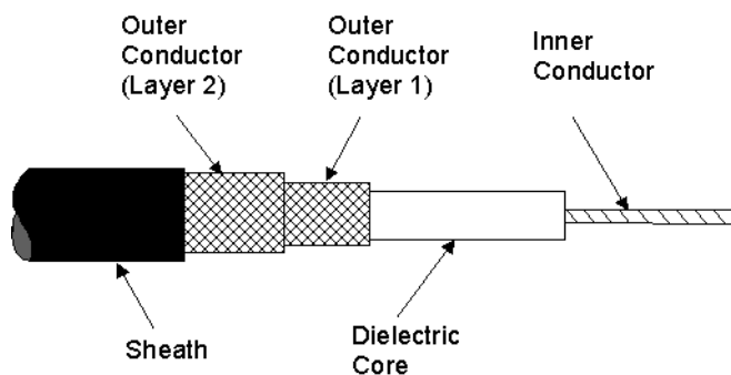
Figure 1. Flexbus cable
