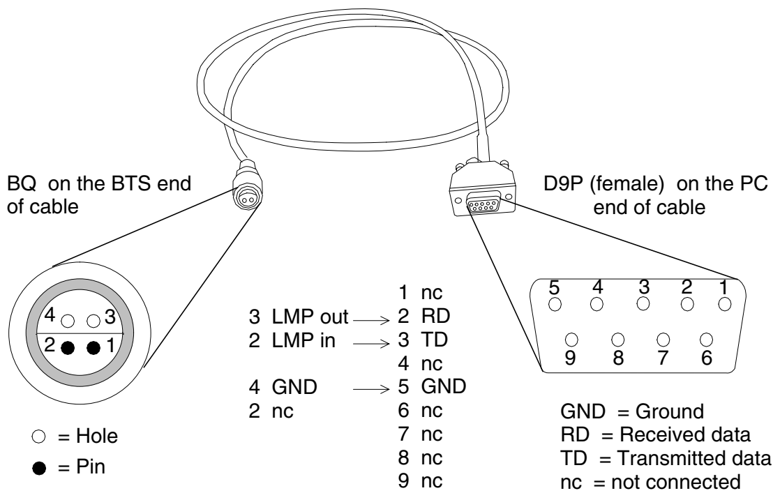
Figure 3. LMP cable and connectors
