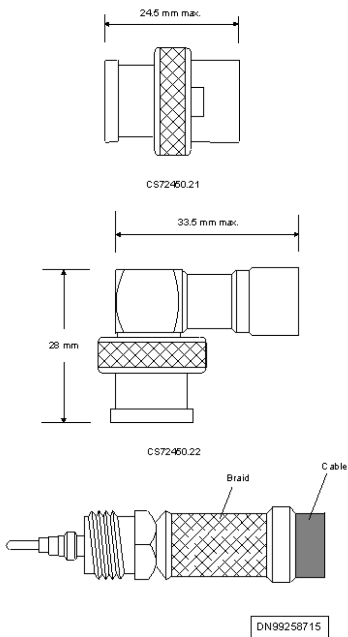
Figure 2. TNC connectors
