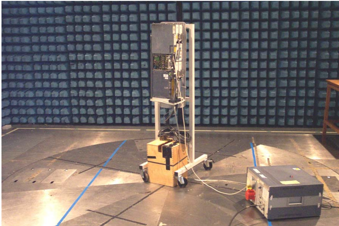
Photograph No 4 – Conducted Emissions – Configuration 5
