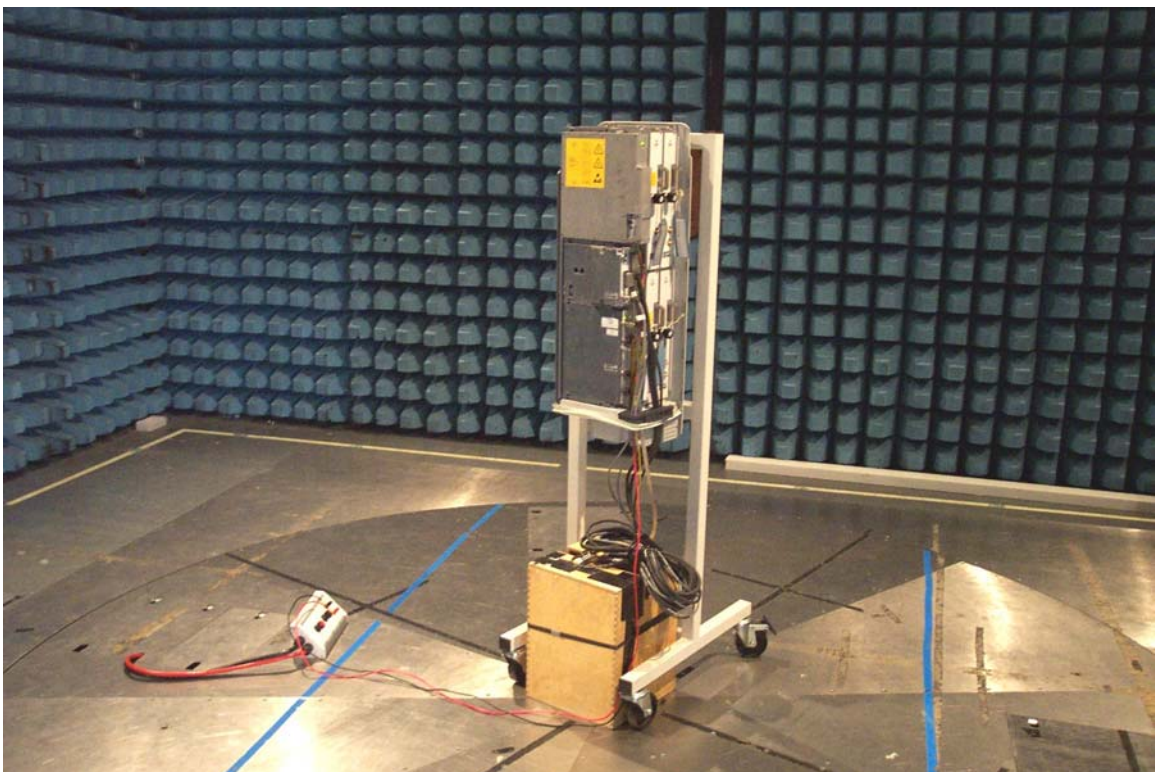
Photograph No 2 – Radiated Emissions – Configurations 1b, 2, 4a and 4b
