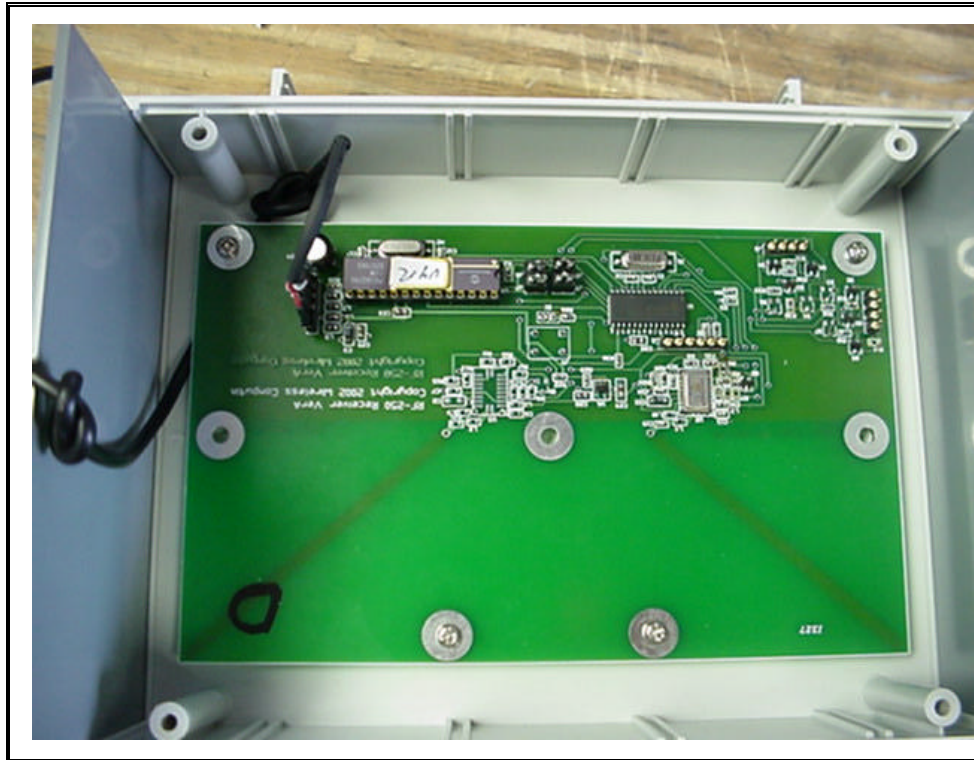
Main Board – Up View
