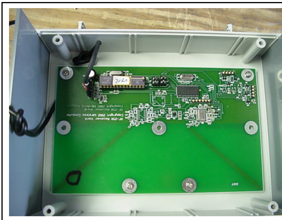
Internal – Bottom View
