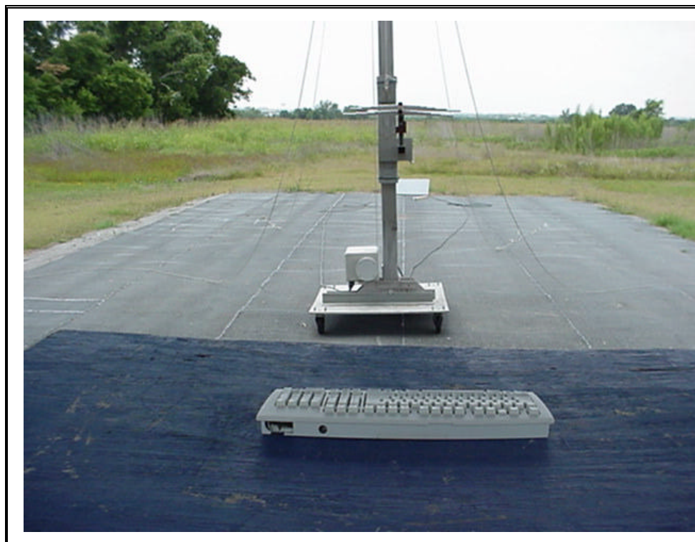
Radiated Emission – Back View
