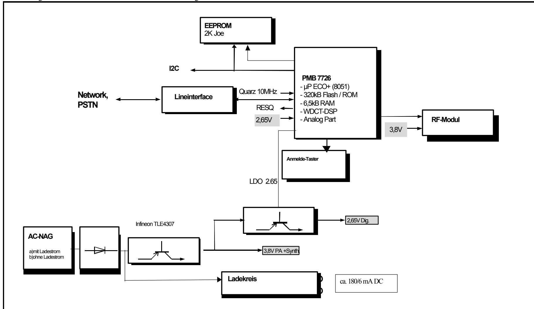
Gigaset 4010 WDCT standard base station block diagram
