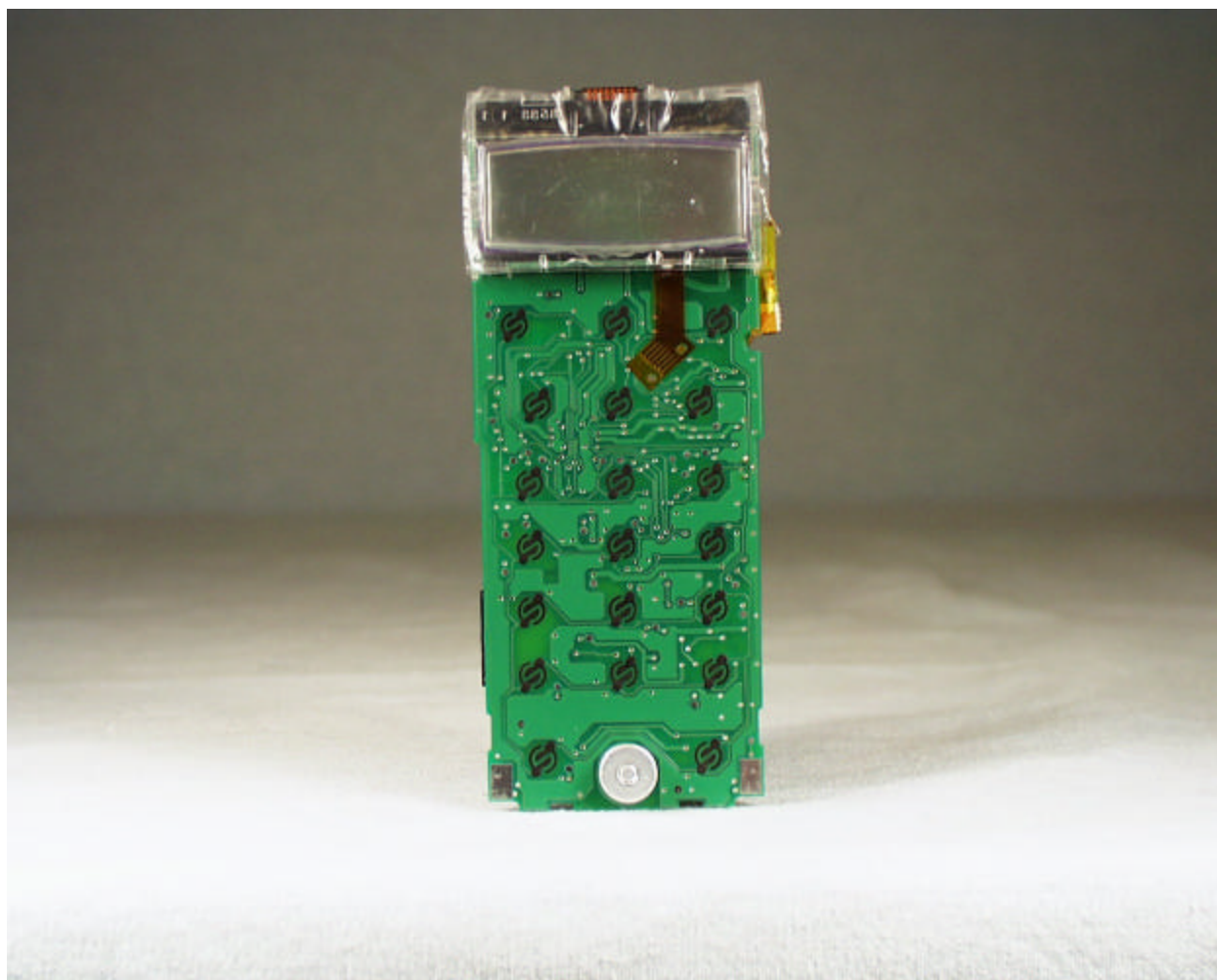
Inside View - Side A - Handset (without keypad)
