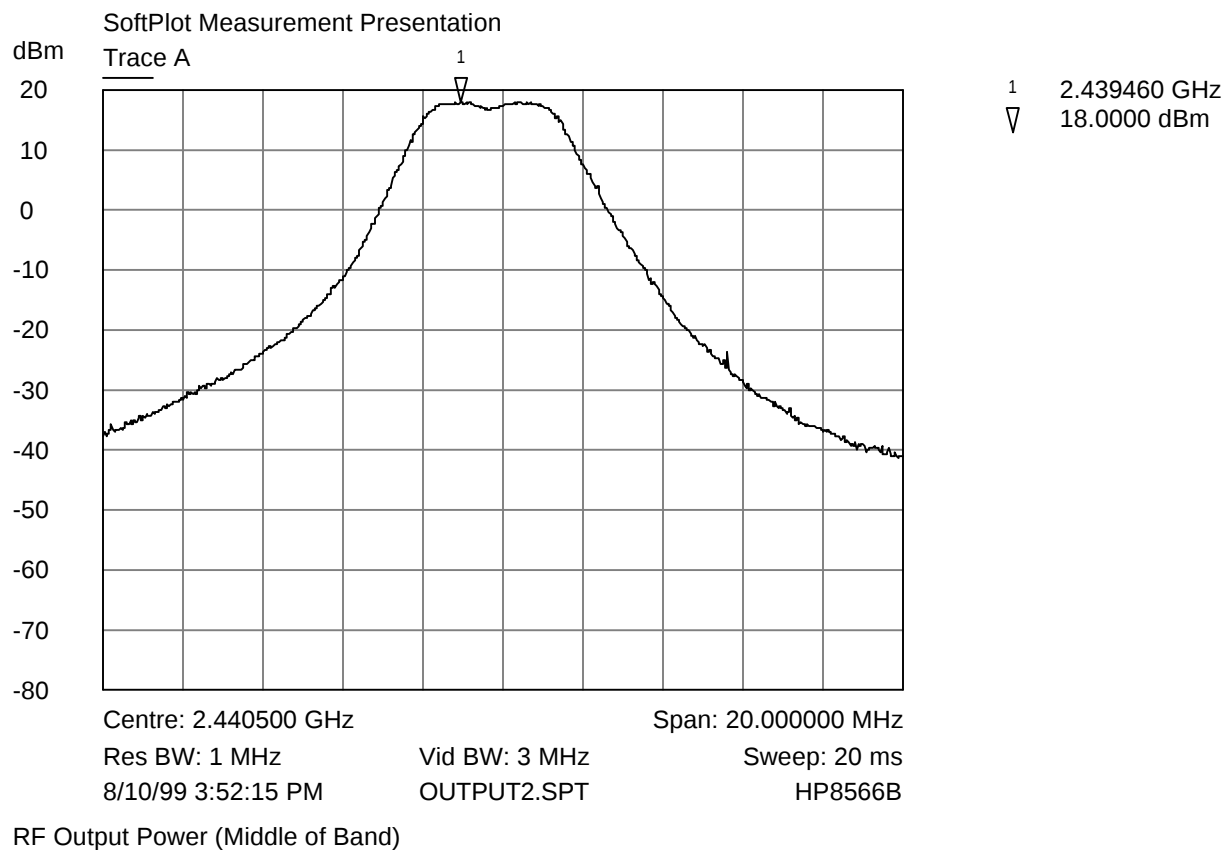
Peak Output Power Plot - Base Station (Middle Channel)
