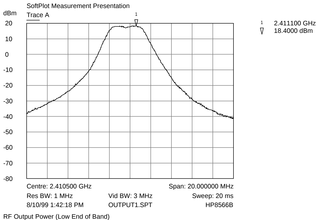
Peak Output Power Plot – Base Station (Low Channel)
