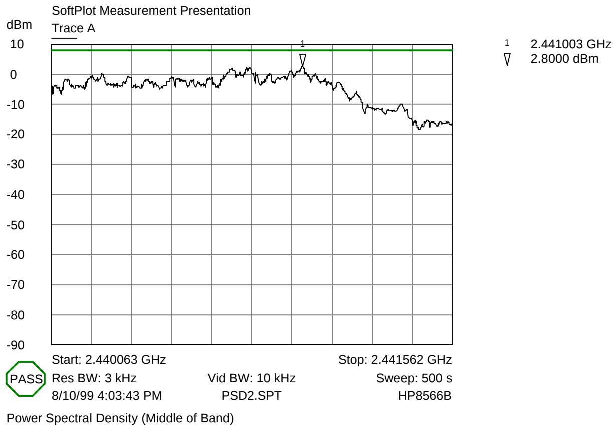
Power Spectral Density Plot - Base Station (Middle Channel)
