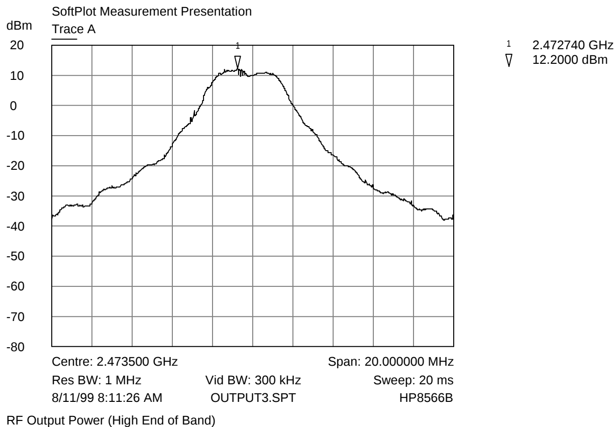
Peak Output Power Plot - Handset (High Channel)
