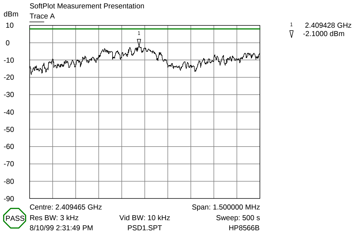
Power Spectral Density Plot - Handset (Low Channel)
