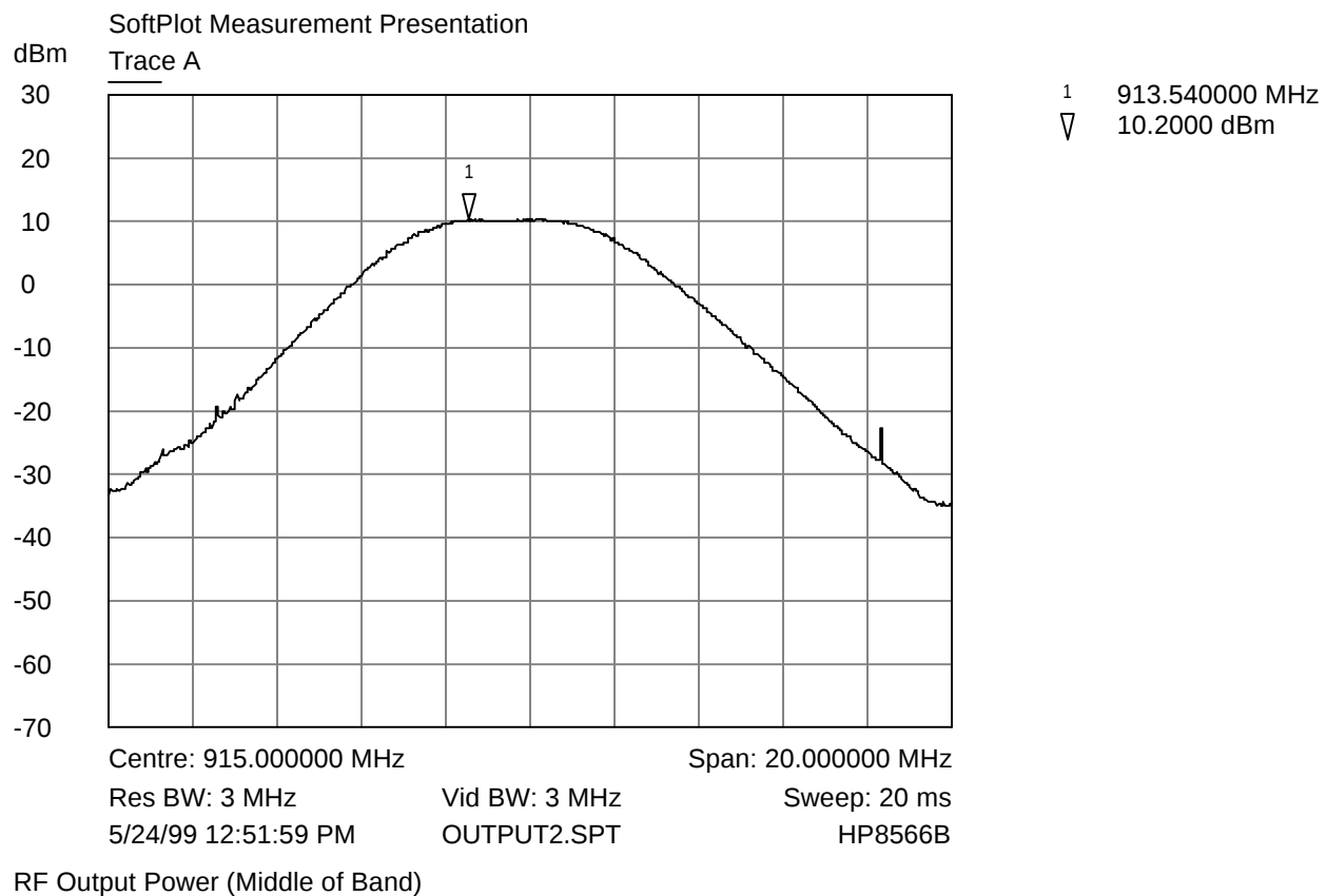
Power Output Plot - Handset (Middle Channel)
