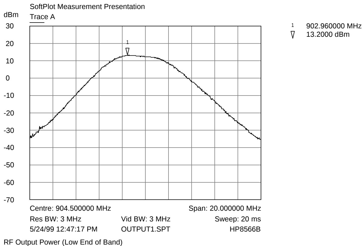
Power Output Plot - Handset (Low Channel)
