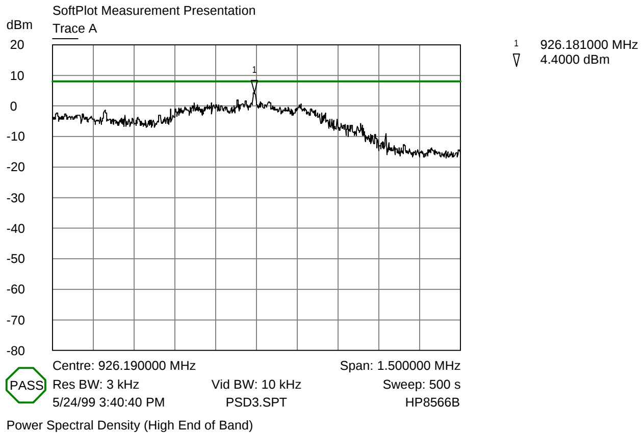
Power Spectral Density Plot - Base Station (High Channel)
