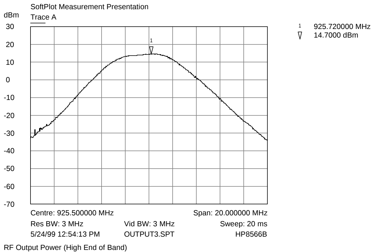
Power Output Plot - Handset (High Channel)
