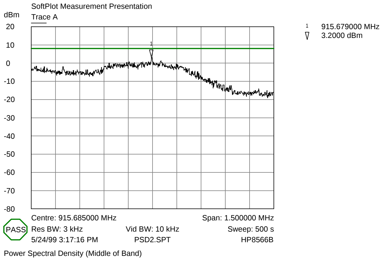
Power Spectral Density Plot - Base Station (Middle Channel)
