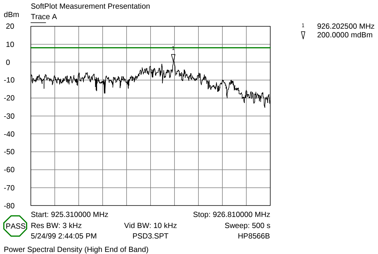
Power Spectral Density Plot - Handset (High Channel)
