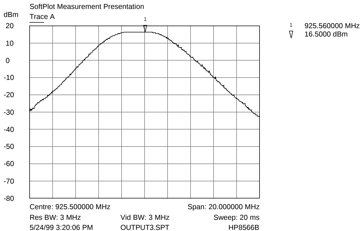
Power Output Plot - Base Station (High Channel)
