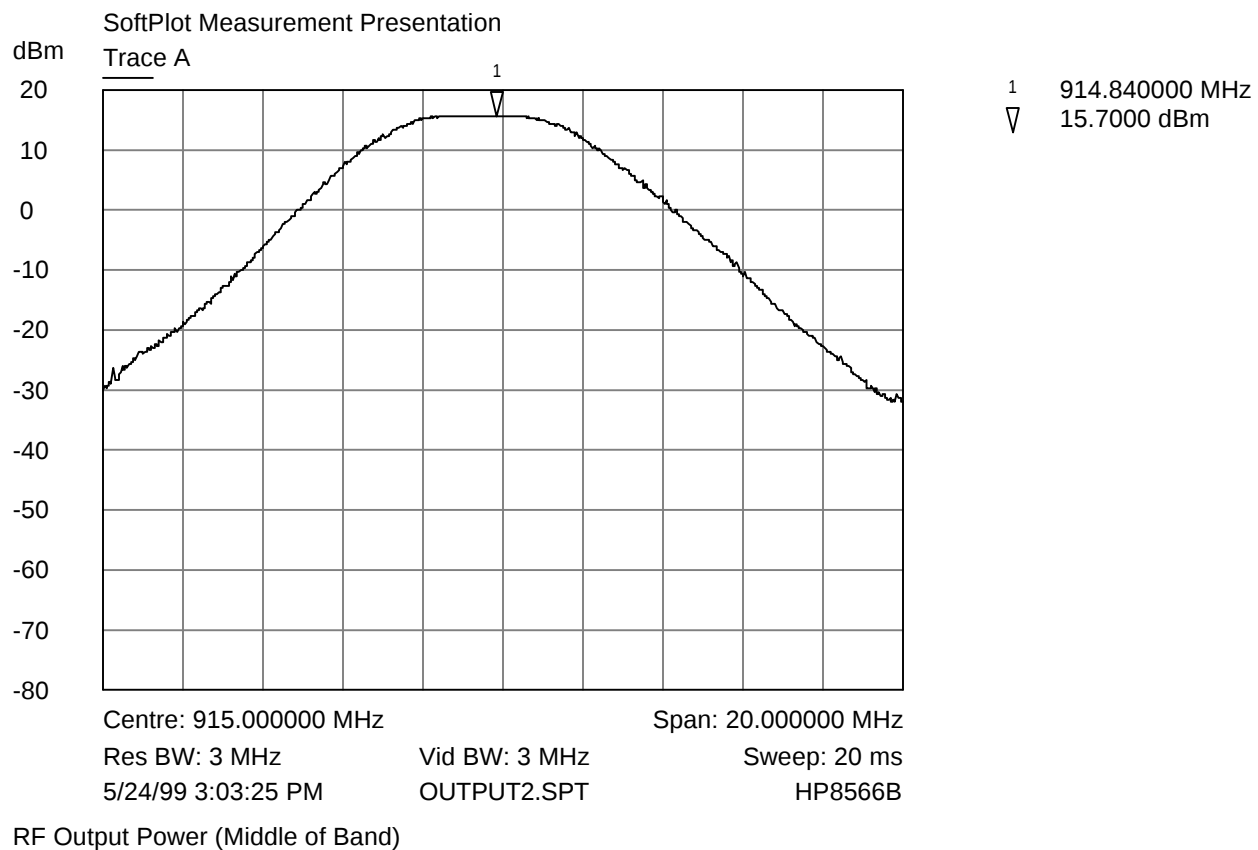
Power Output Plot - Base Station (Middle Channel)
