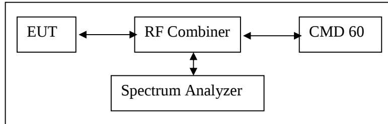
Figure 13: CMD60 and Spectrum Analyzer Test Setup
