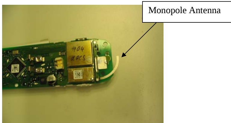
Figure 25: MS Antenna
