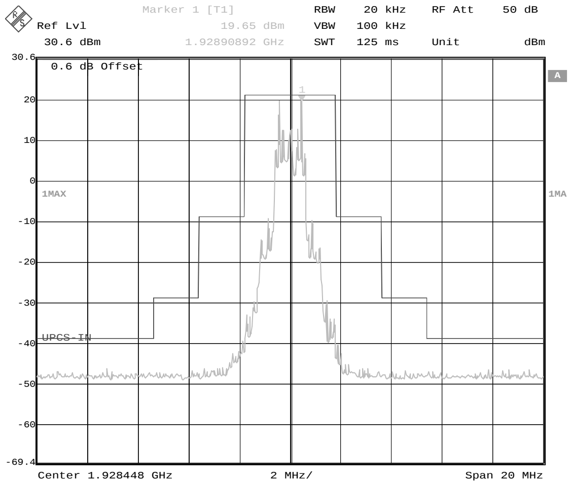
Figure 12: In-Band Spurious Emission of MS at CH5
