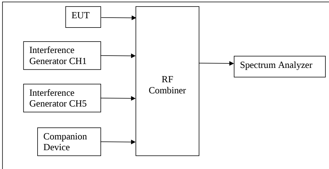
Figure 20: Test Setup for LIC Measurement of MS
