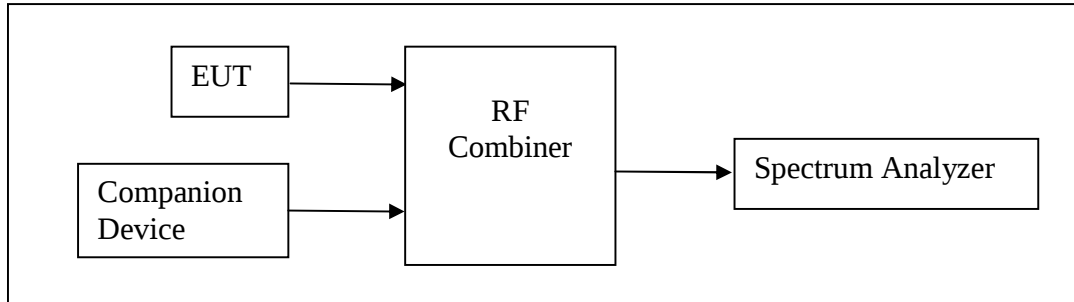
Figure 18: Test Setup for System Acknowledgement of MS
