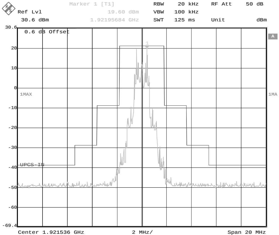
Figure 10: In-Band Spurious Emission of MS at CH1
