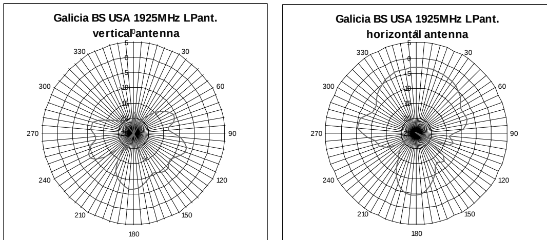
Figure 11: Antenna Diagram of BS PCB Antenna at CH3
