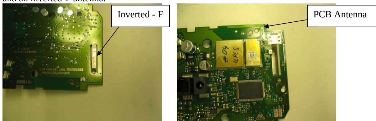
Figure 28: BS Antennae
