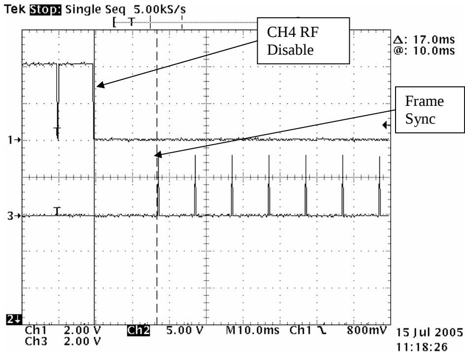
Figure 20: RF Disable and Frame Sync for Monitoring Time on BS
