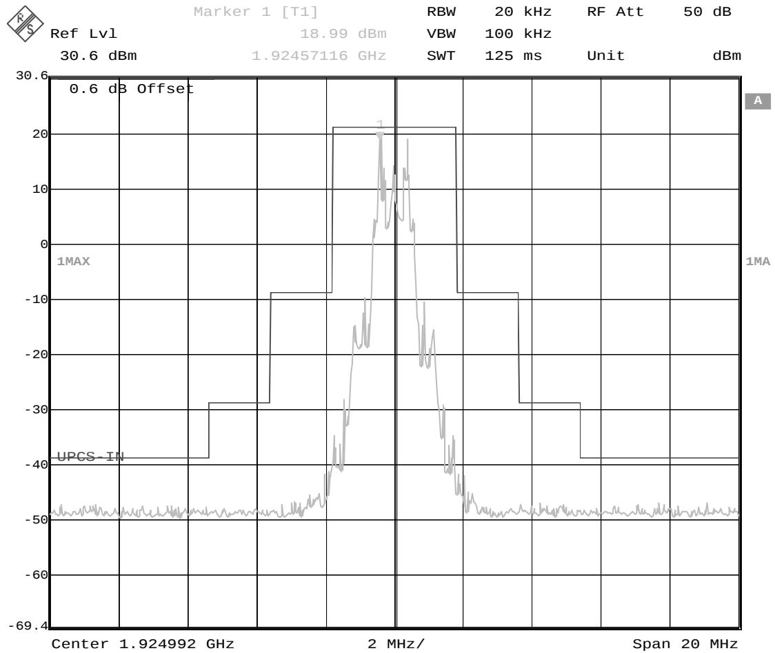
Figure 15: In-Band Spurious Emission of BS at CH3
