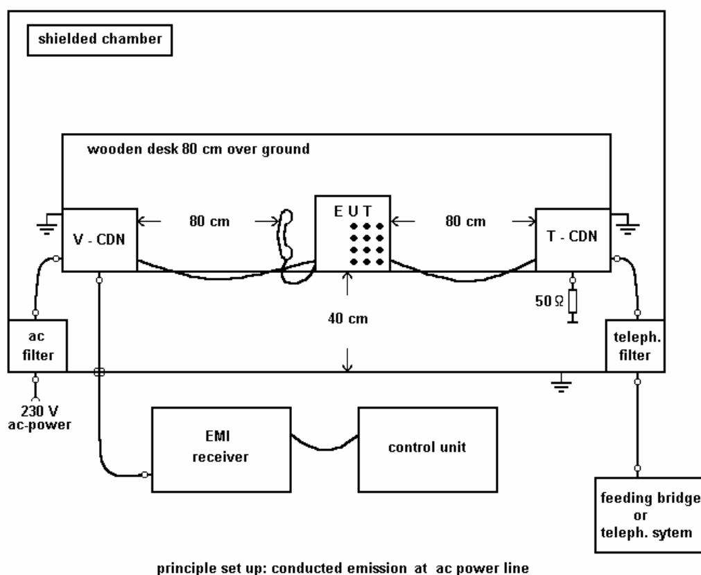
Figure 1: Test Setup for Conducted Emissions
