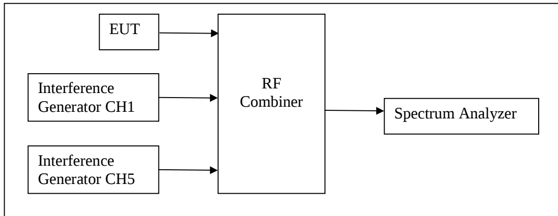
Figure 25: Test Setup for LIC Measurement of BS
