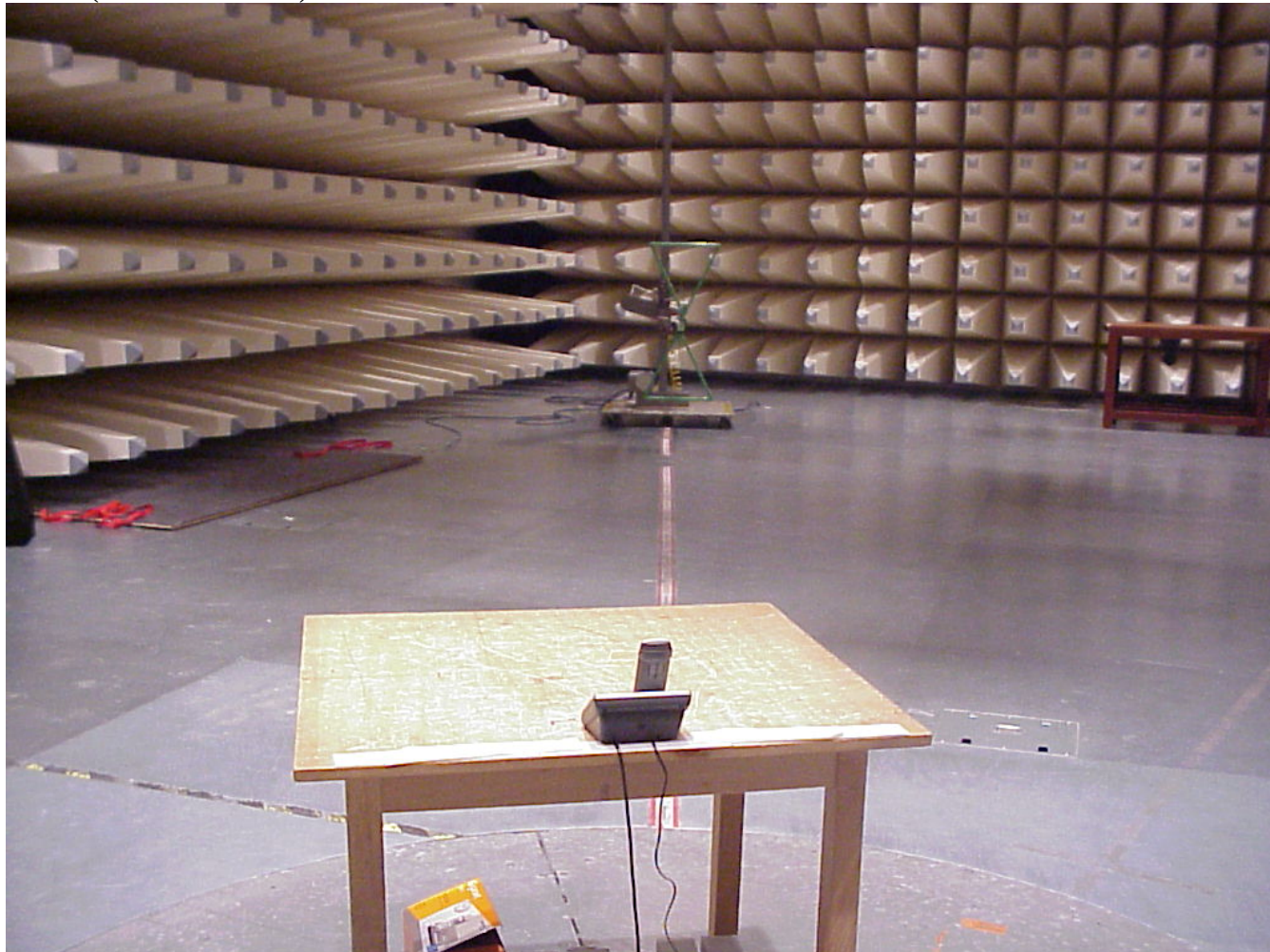
Photo 2 (Radiated Emissions):
