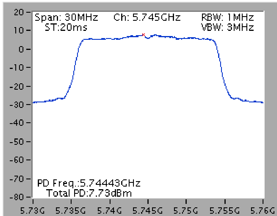
Power Density Plot on Configuration IEEE 802.11ac MCS0/Nss1 VHT20 / Ant. 1 + Ant. 2 / 5745 MHz
