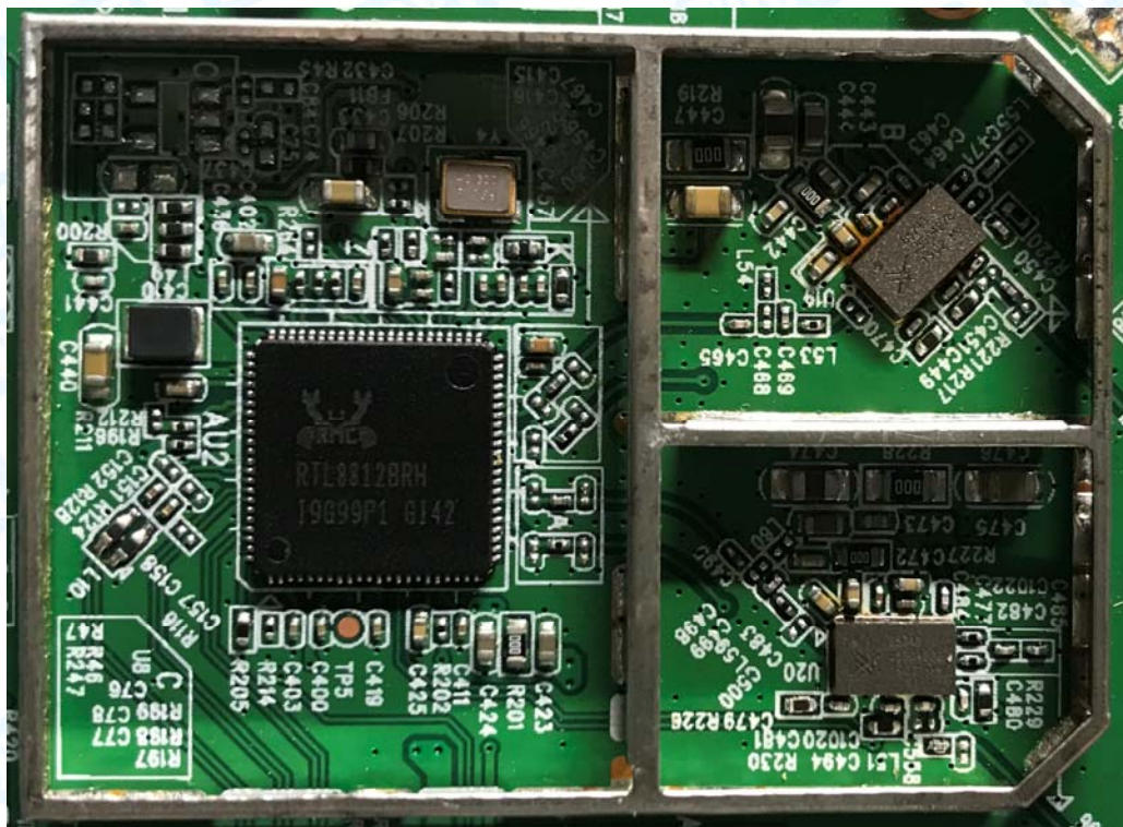
Photo 19 Appearance of PCB
