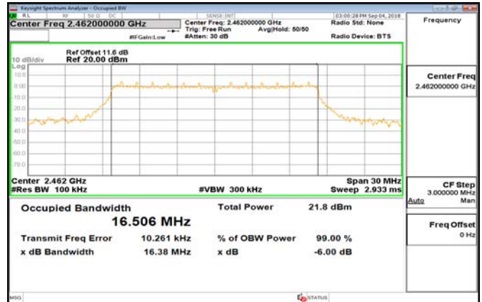
6dB Band Width Test Data CH-High (2462MHz)
