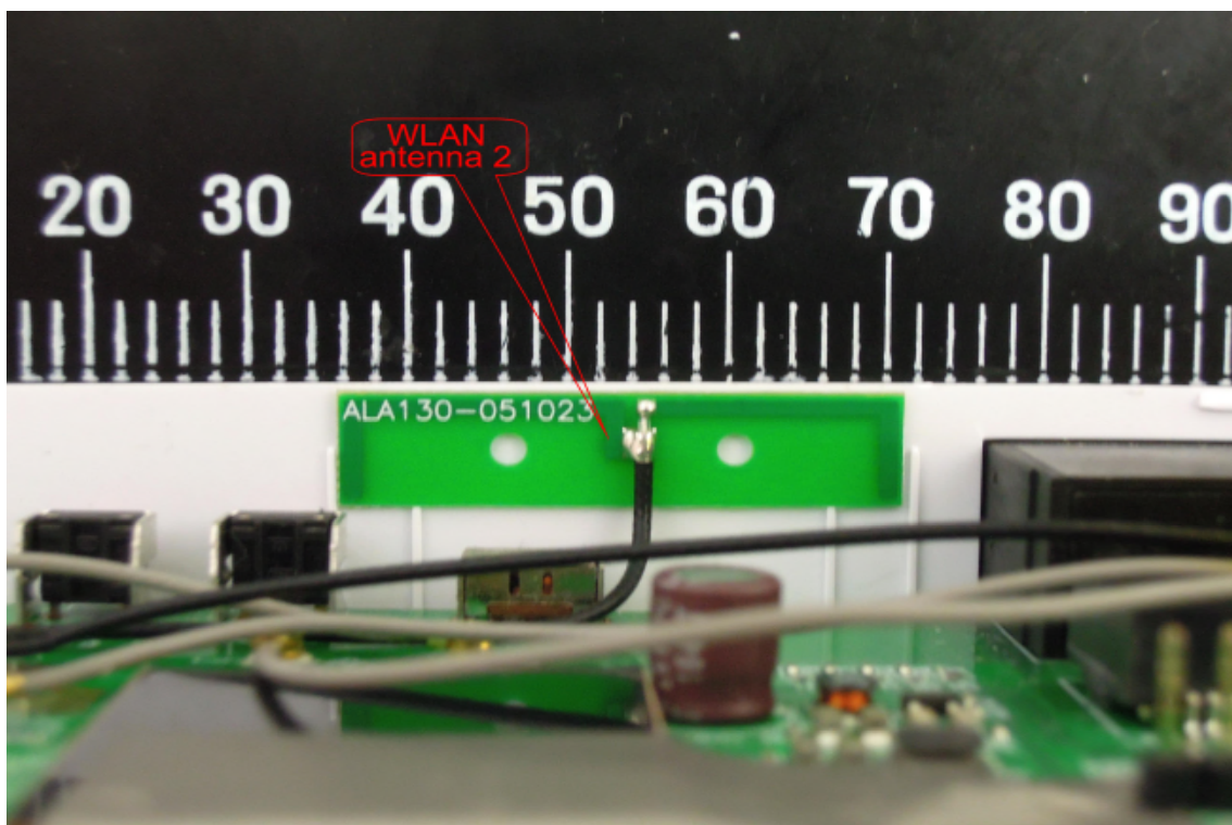
WLAN Antenna-2
