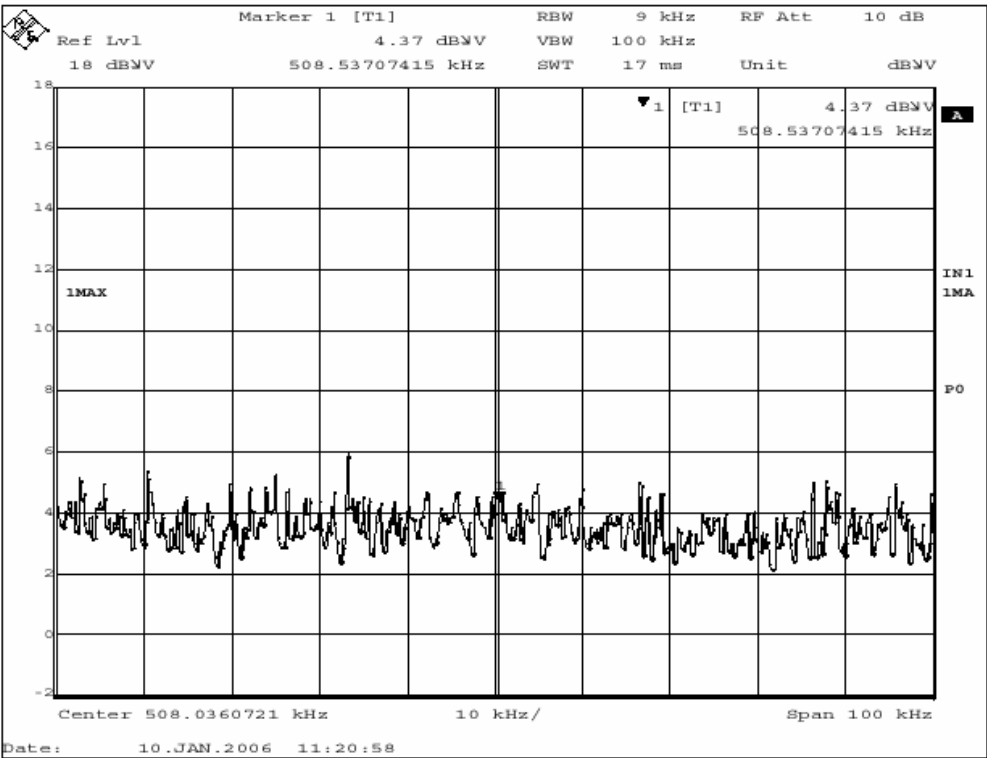
Figure 10 - Transmit ON, 3m Measurement Distance, uncorrected
