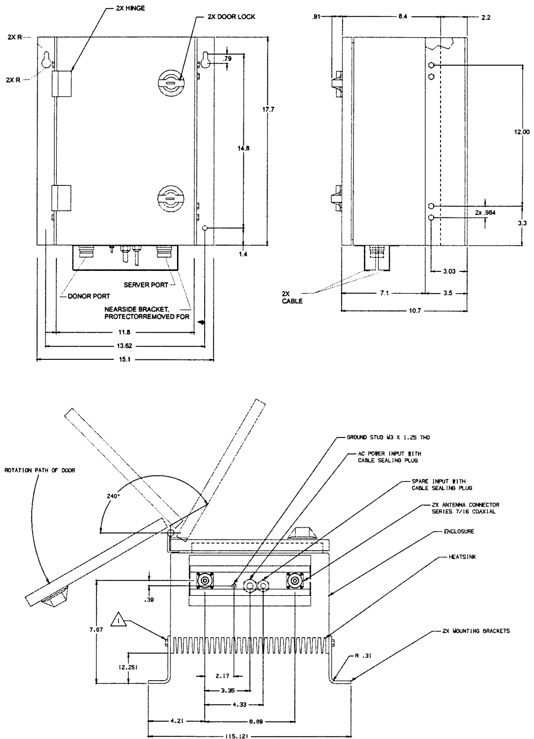
Figure 18. Repeater Dimensions, shown in inches.
