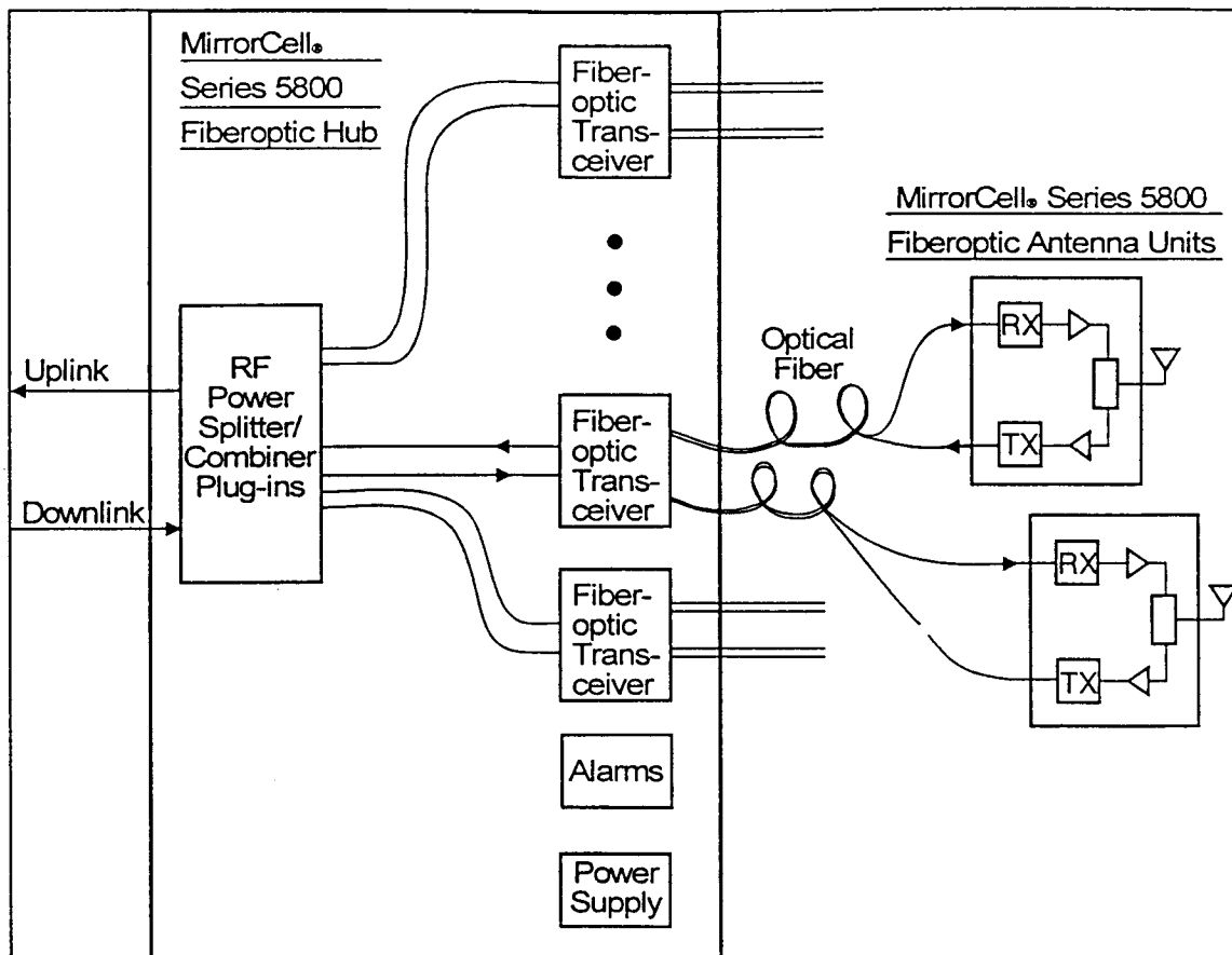
MirrorCell Series 5800 Fiberoptic Link between the Hub and the antenna unit.
