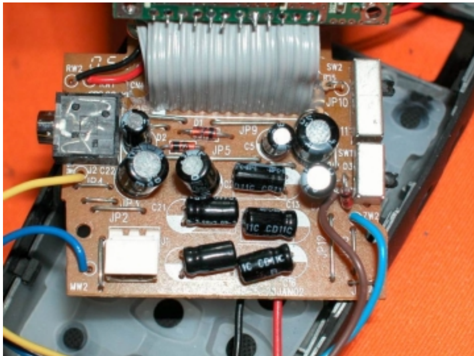
Handset another PCB comp side (View 1)
