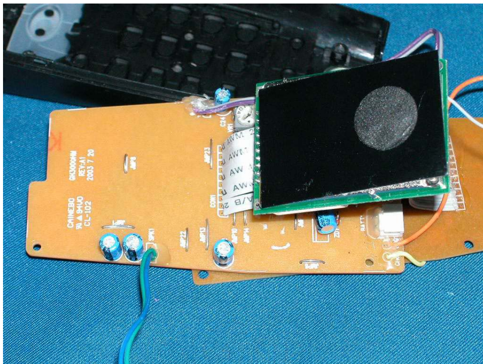
Handset Main PCB front side (View 2)
