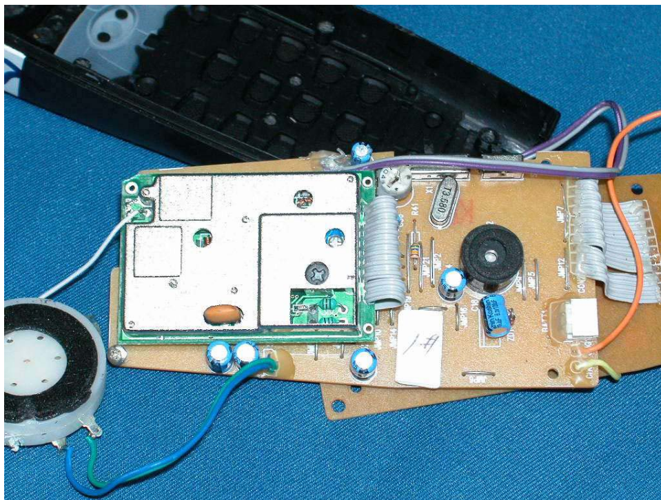
Handset Main PCB front side (View 1)
