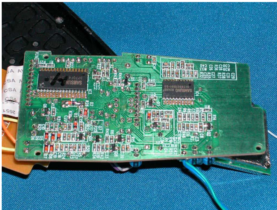
Handset Main PCB rear side
