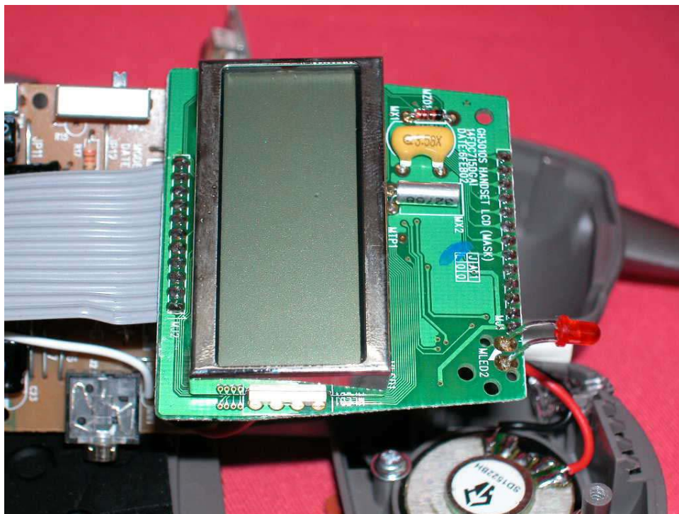
Handset Main PCB display front side
