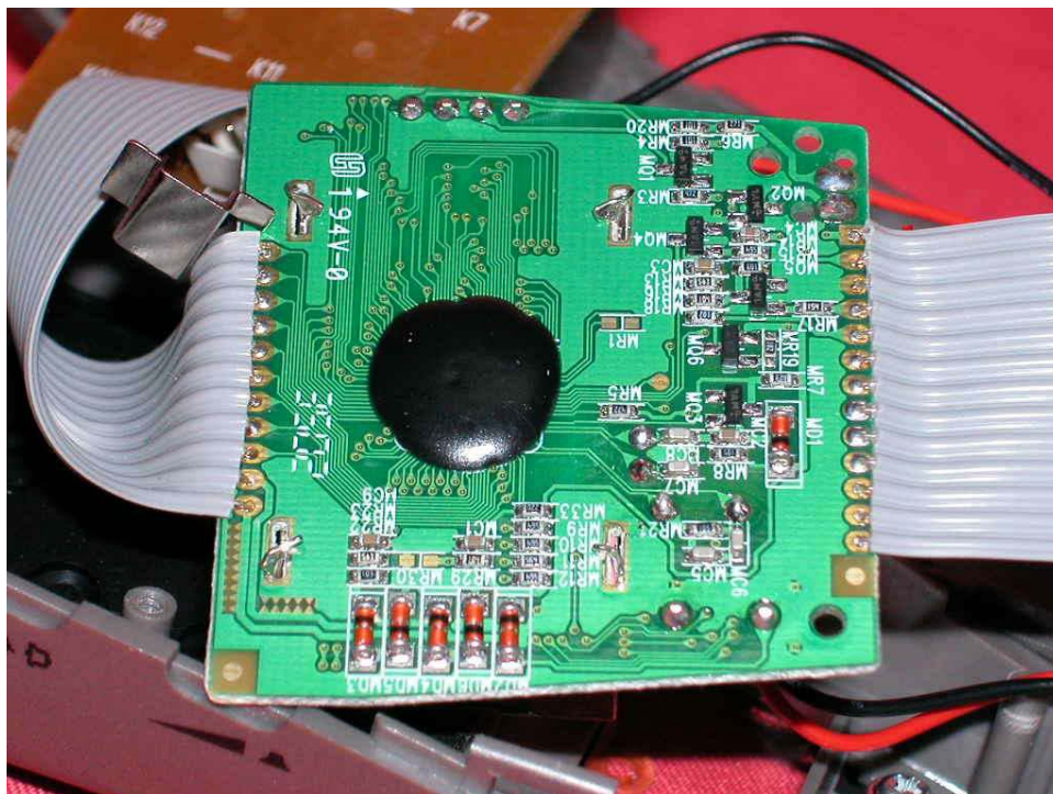
Handset Main PCB display rear side
