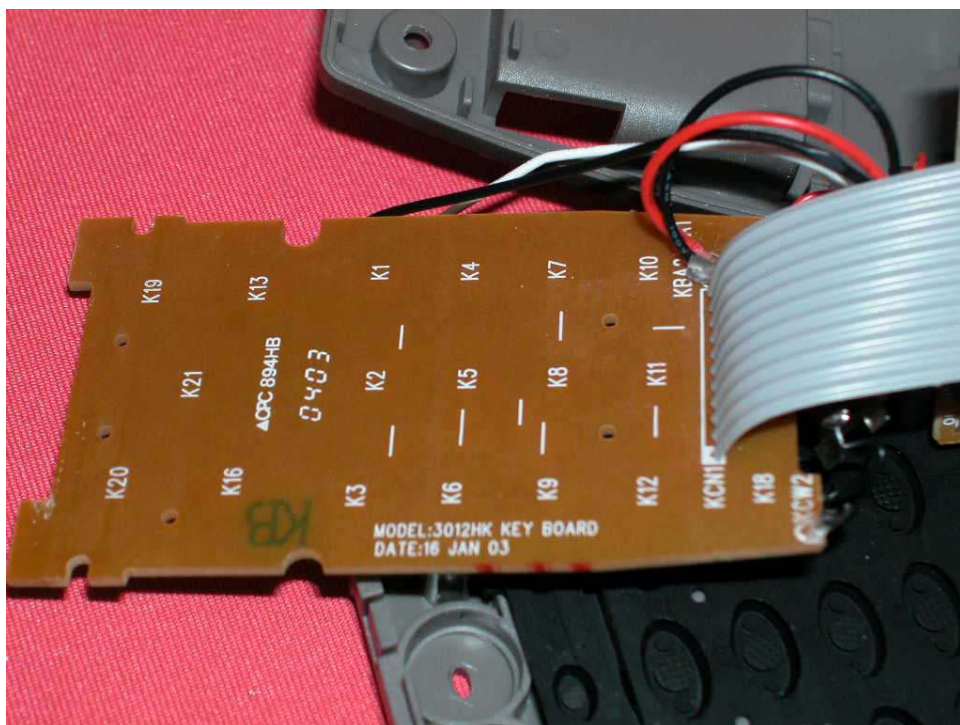
Handset keypad side rear side (View 1)
