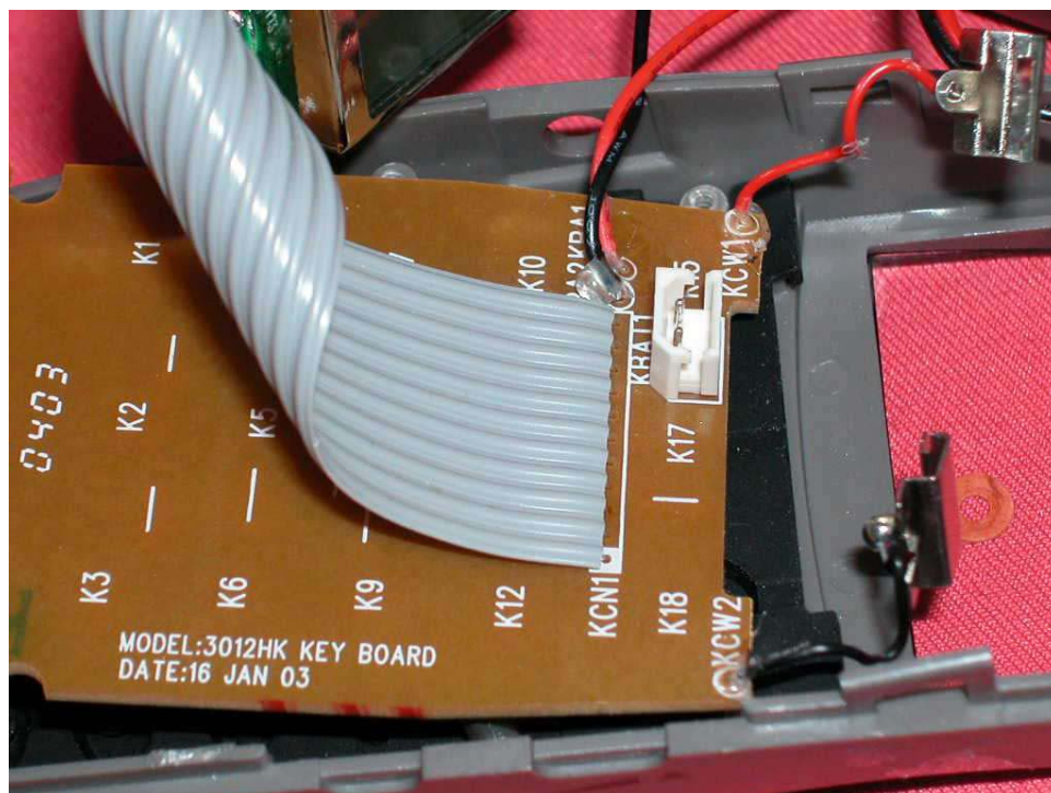
Handset keypad side rear side (View 2)
