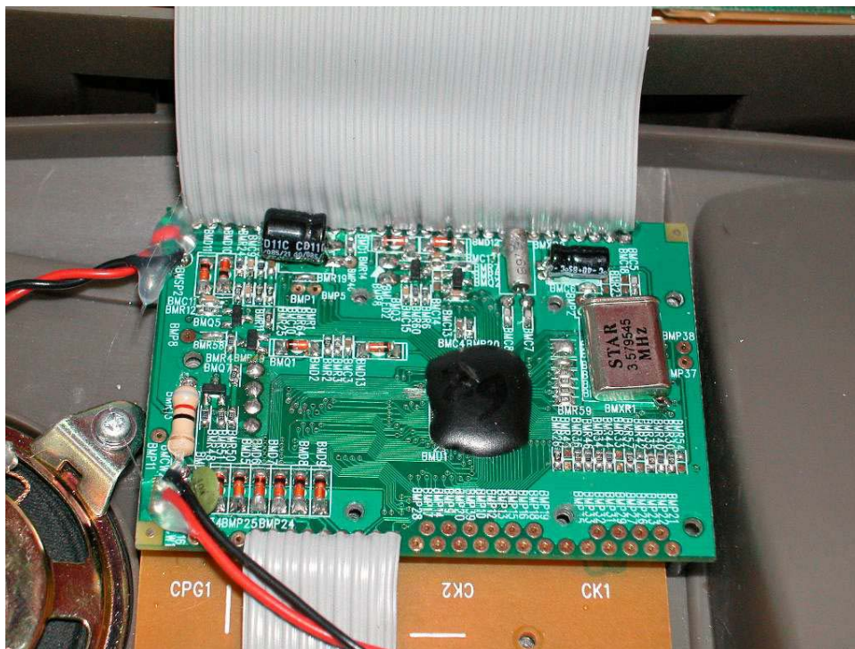
Base LCD display PCB comp side
