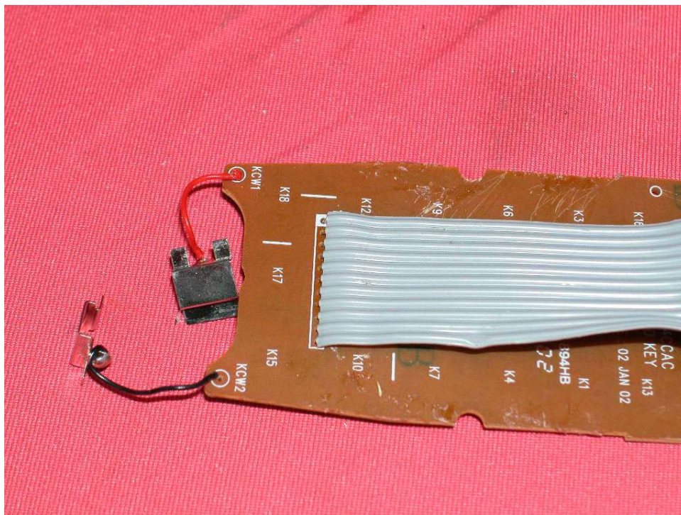
Handset keypad PCB rear side (view 2)
