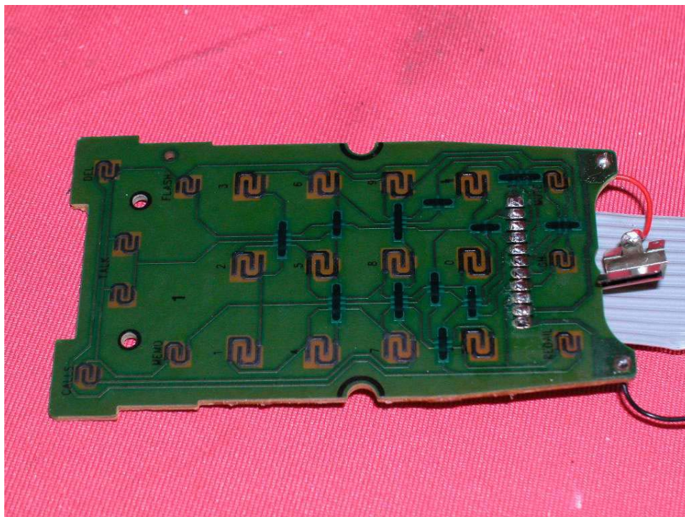
Handset keypad PCB front side
