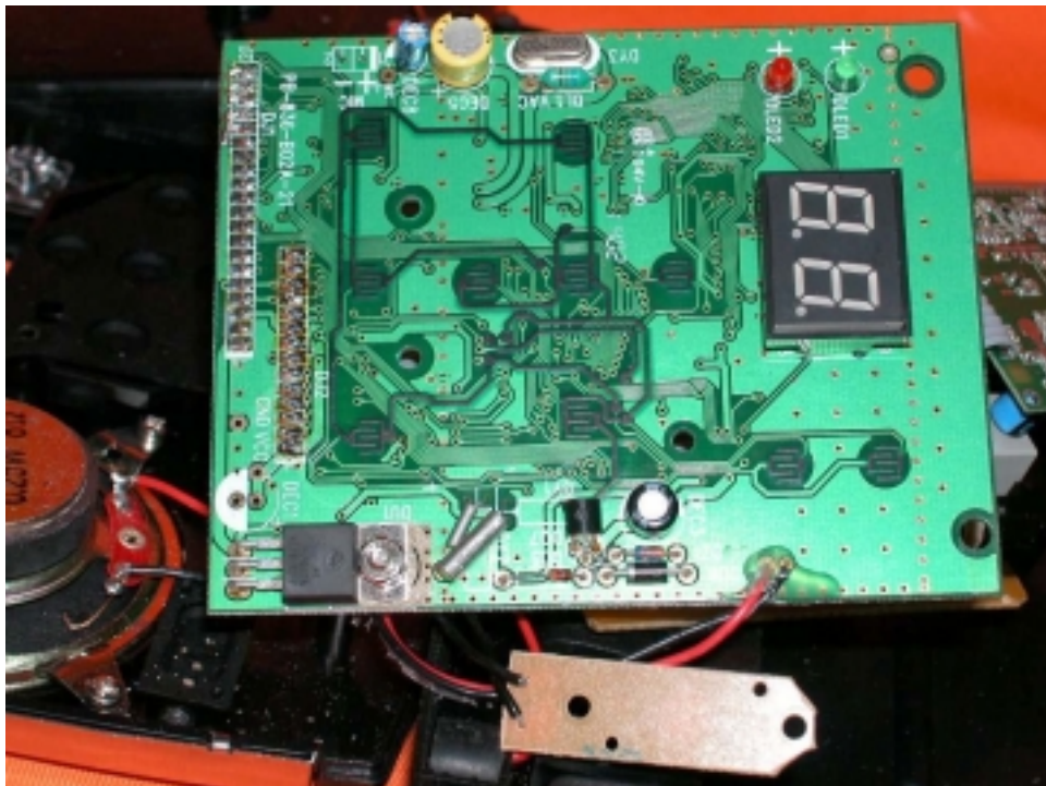
Answer Machine PCB keypad side
