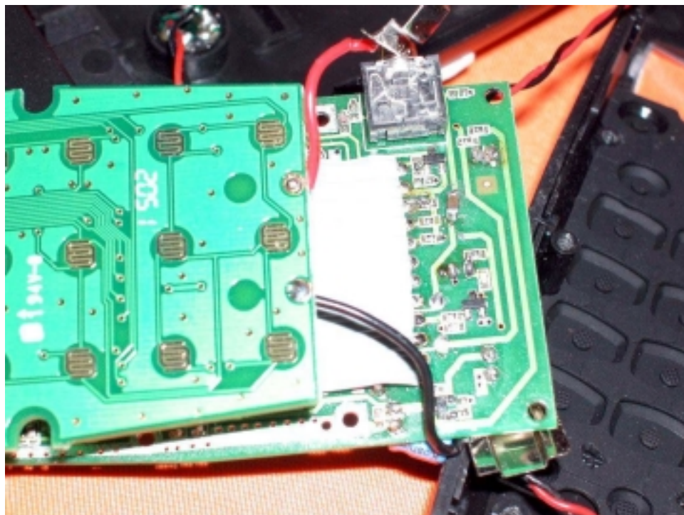
Handset Oscillator PCB solder side (View 2)
