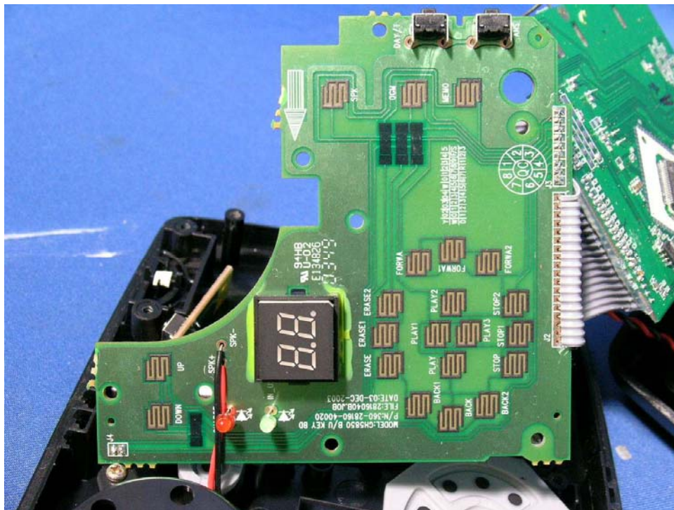
Base DAM PCB front side
