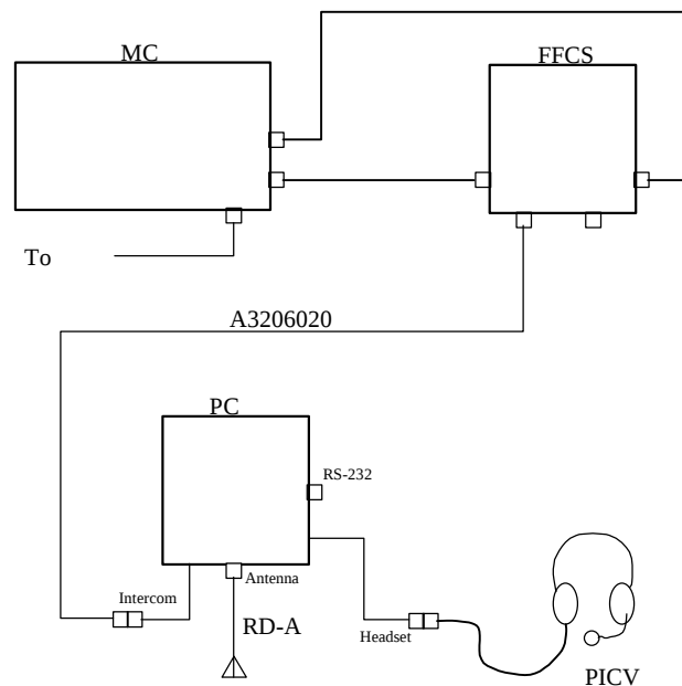
Figure 1. Test Configuration A
