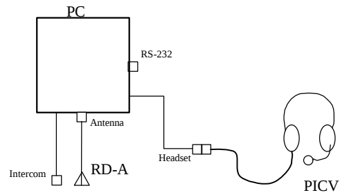
Block Diagram A – Untethered Operation
