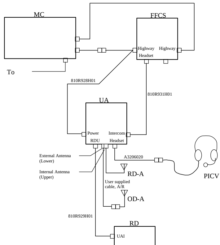
Figure 1. Test Configuration
