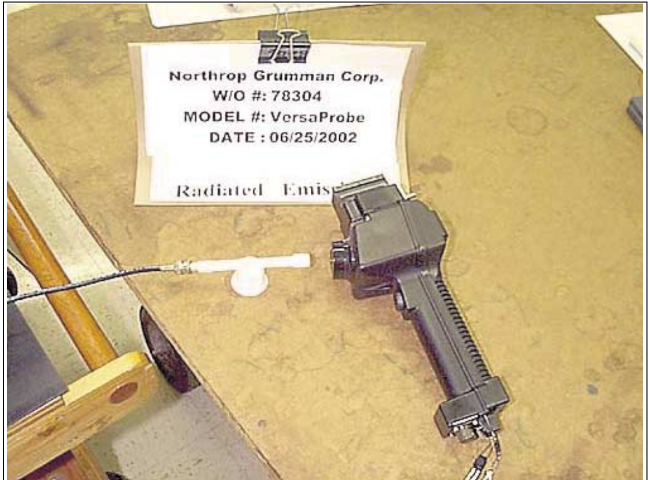
Radiated Emissions - Front View - H-Probe Antenna
