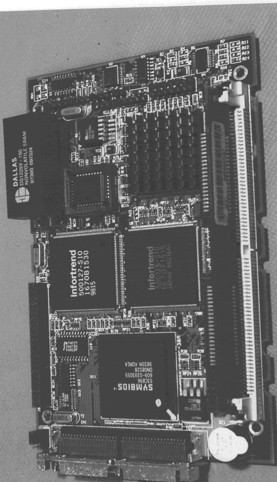
PHOTO 7. EUT COMPONENT SIDE VIEW
