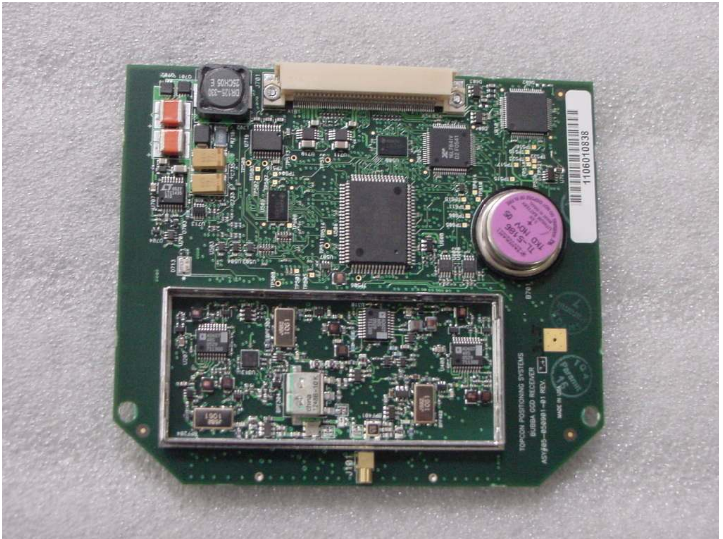
Top of GPS board shield removed
