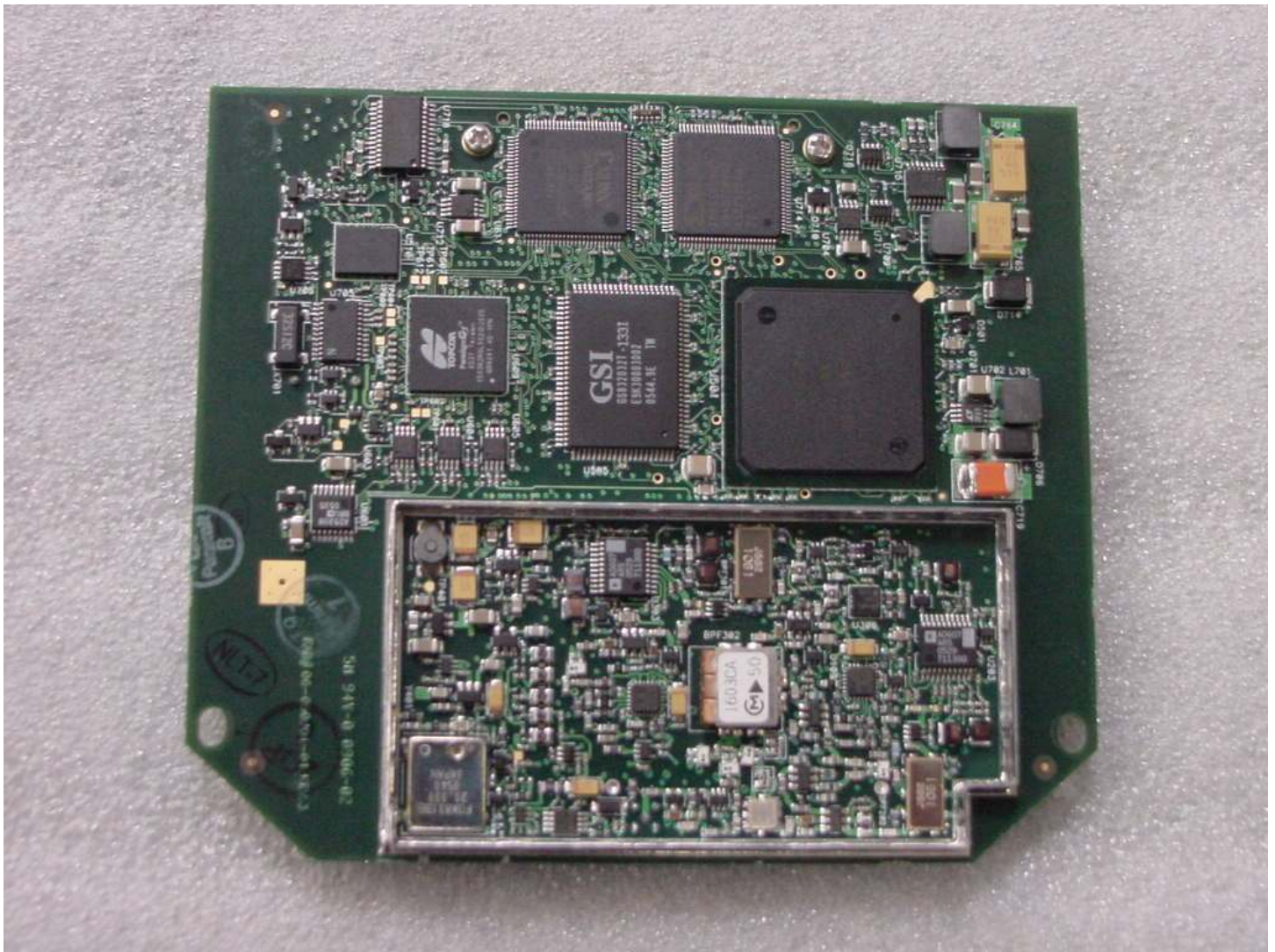
Bottom of GPS board shield removed
