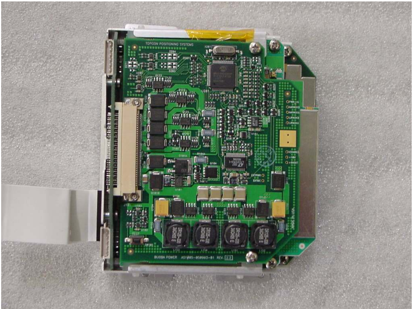
Card cage showing powerboard
