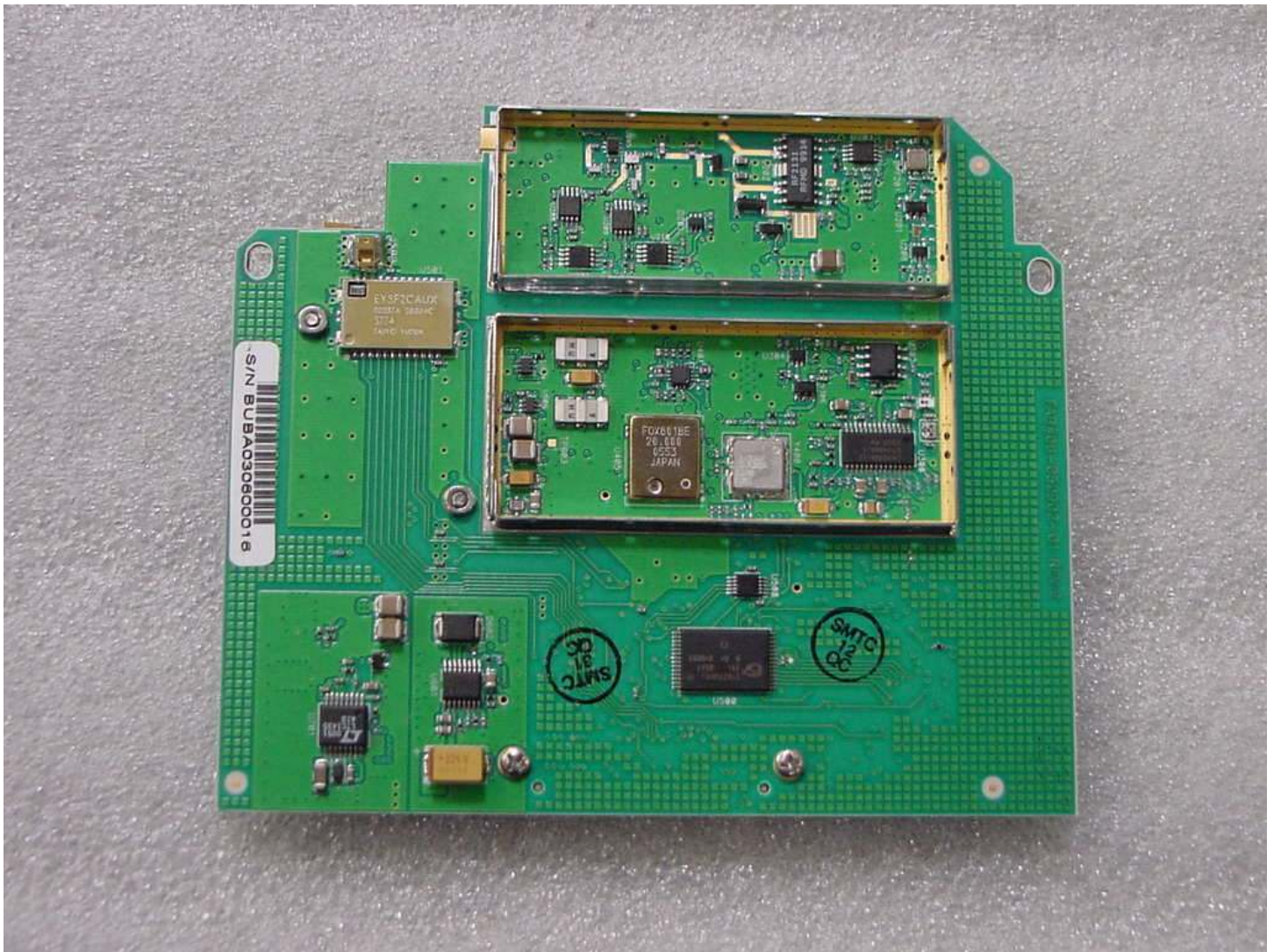
Top of FH915+ modem board shields removed
