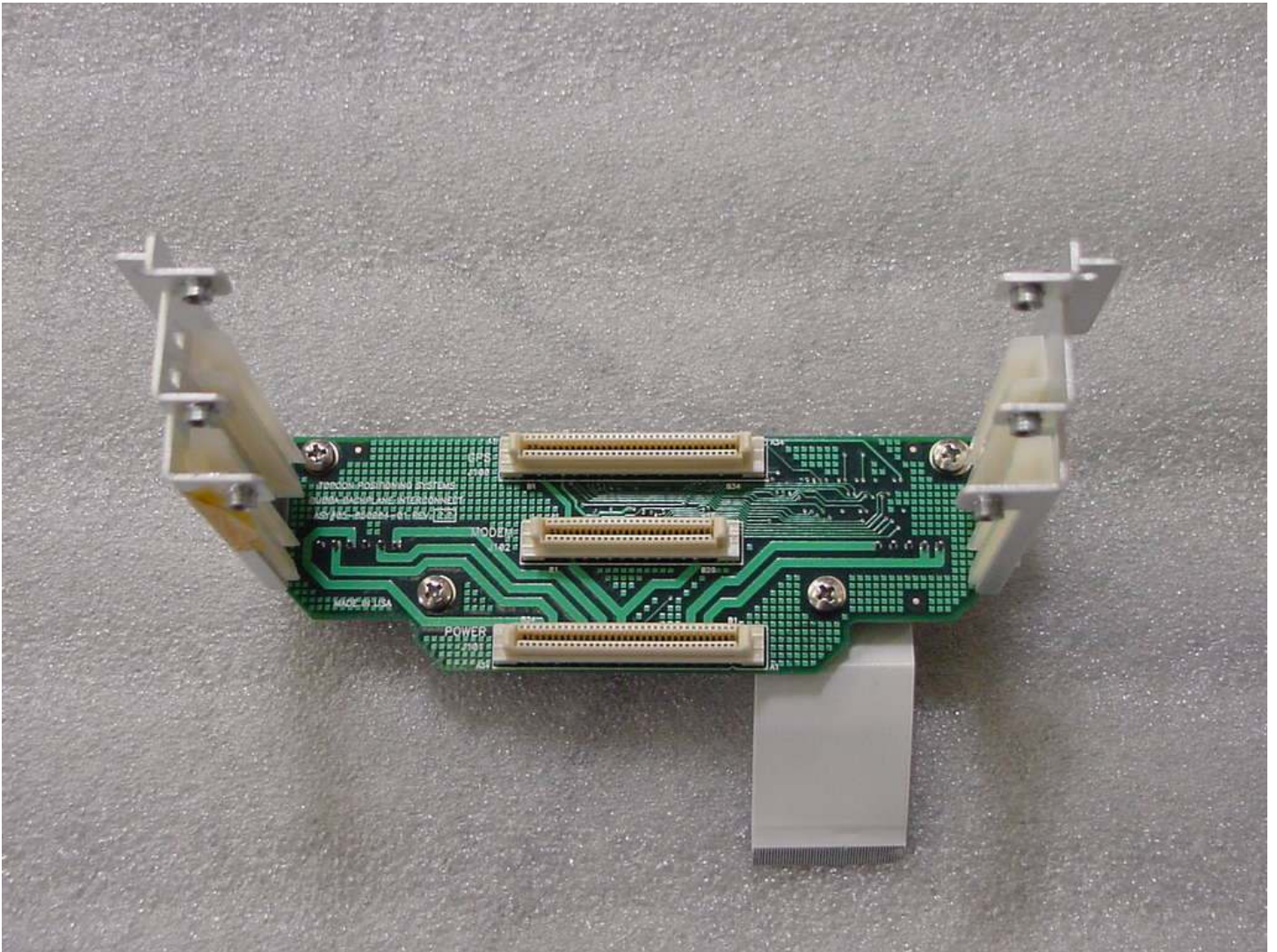
Interconnect board inside card cage
