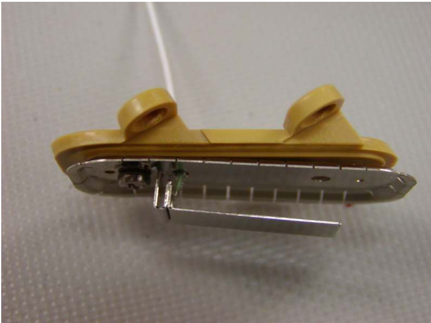
Bluetooth® antenna
