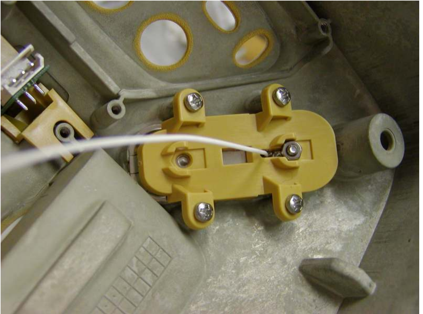
Bluetooth® Antenna placement
