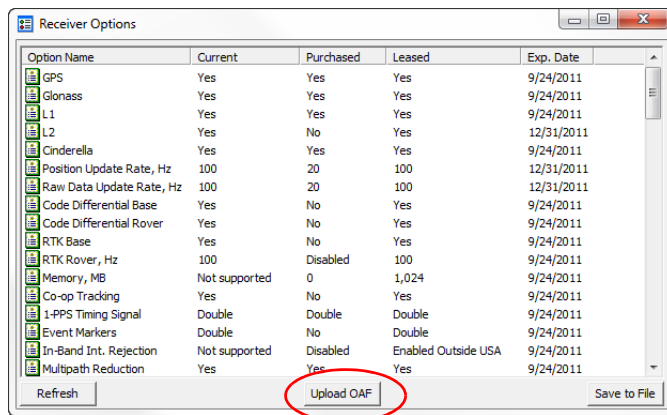
Figure 22: Receiver Options
