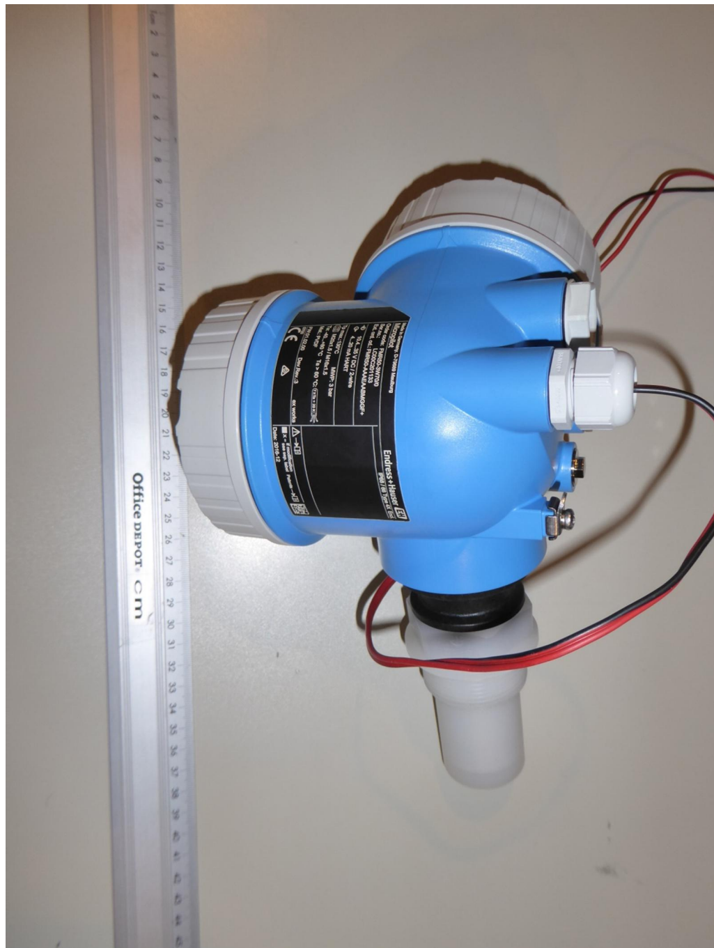
172289_g.JPG: ProToF BTLE-adaptor 2.4 GHz inside FMR50, external view 2
