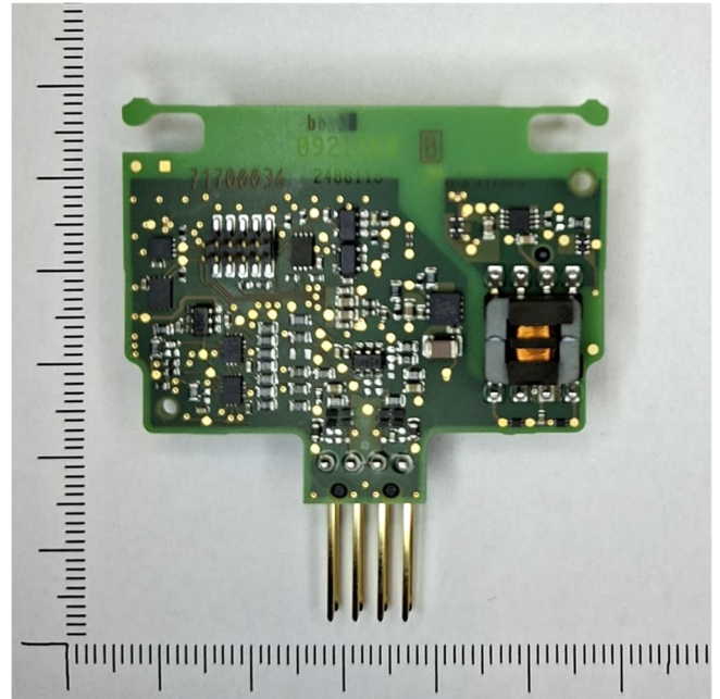
Sensor board - side 2 *
