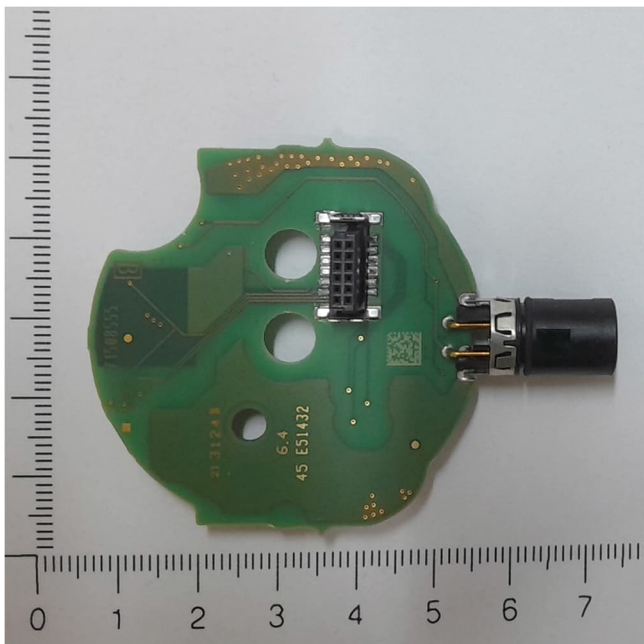
Terminal board - top view *
