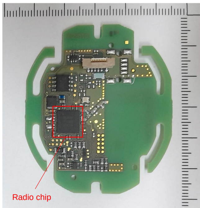
Visualisation board, bottom view *
