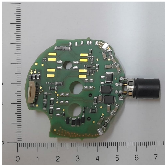
Terminal board - bottom view *
