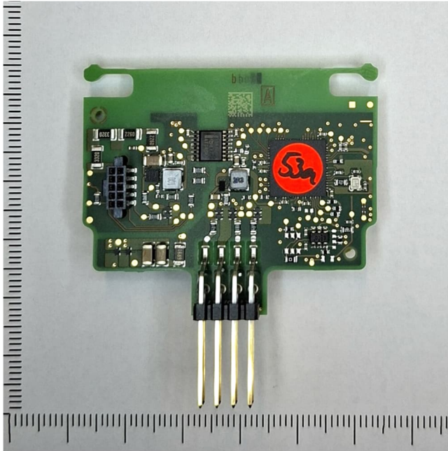
Sensor board - side 1 *
