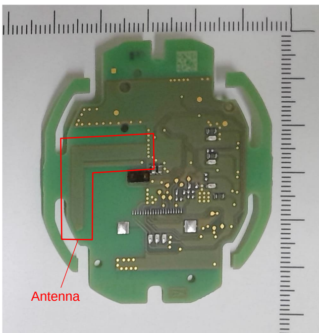
Visualisation board, top view *
