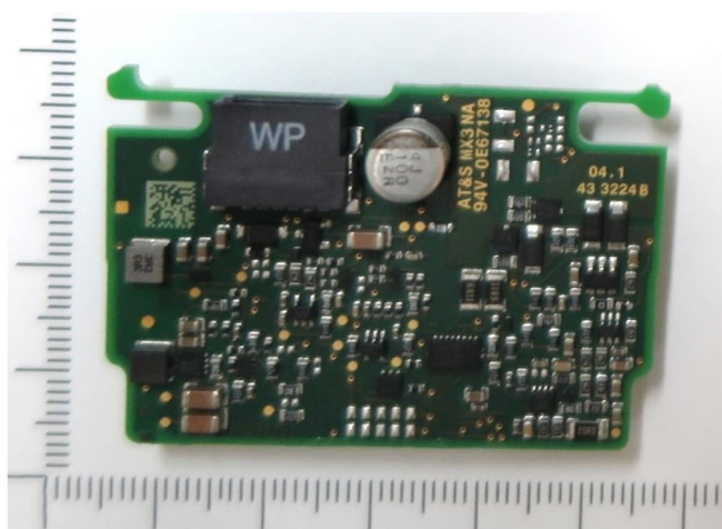
Mainboard - side 2 *
