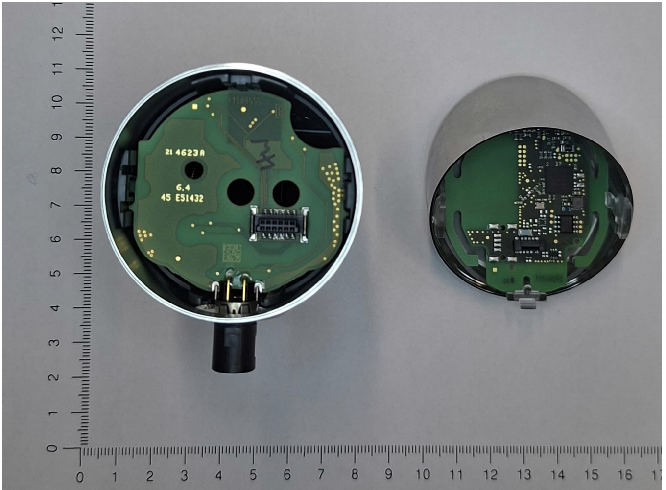
Housing with display *
