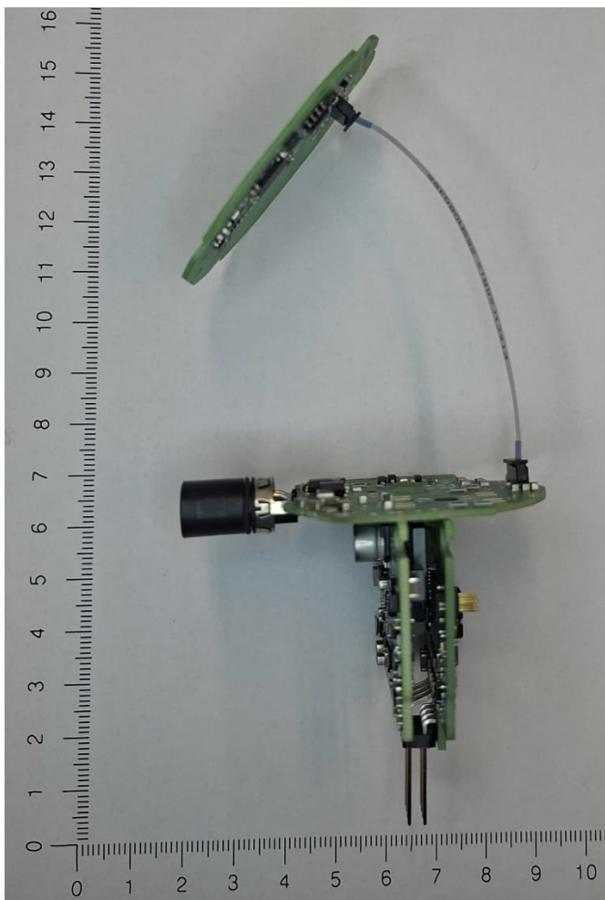
All PCBs connected - view 1 *
