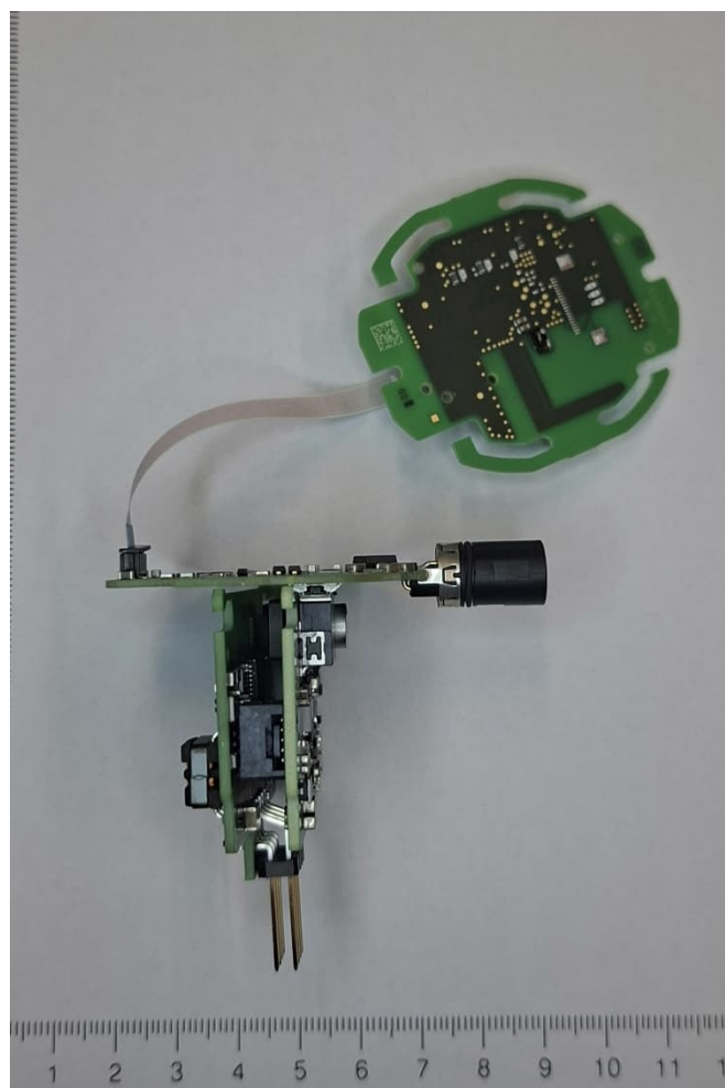
All PCBs connected - view 2 *
