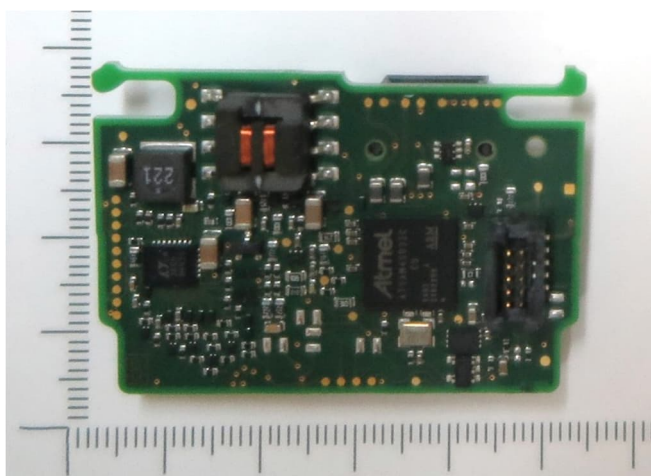
Mainboard - side 1 *
