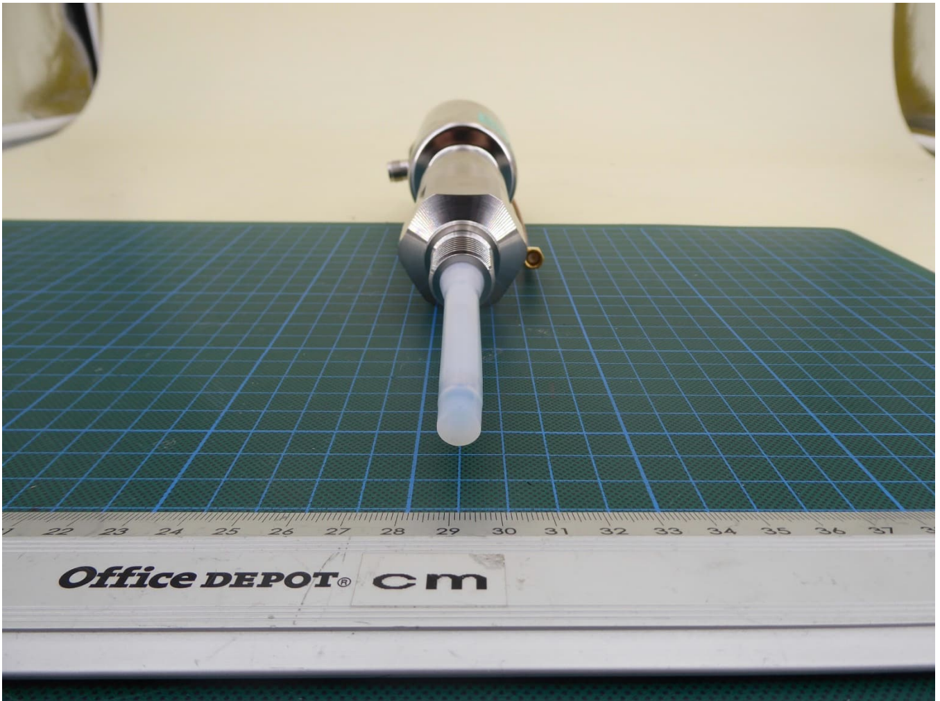
Conducted EUT – side view 4
