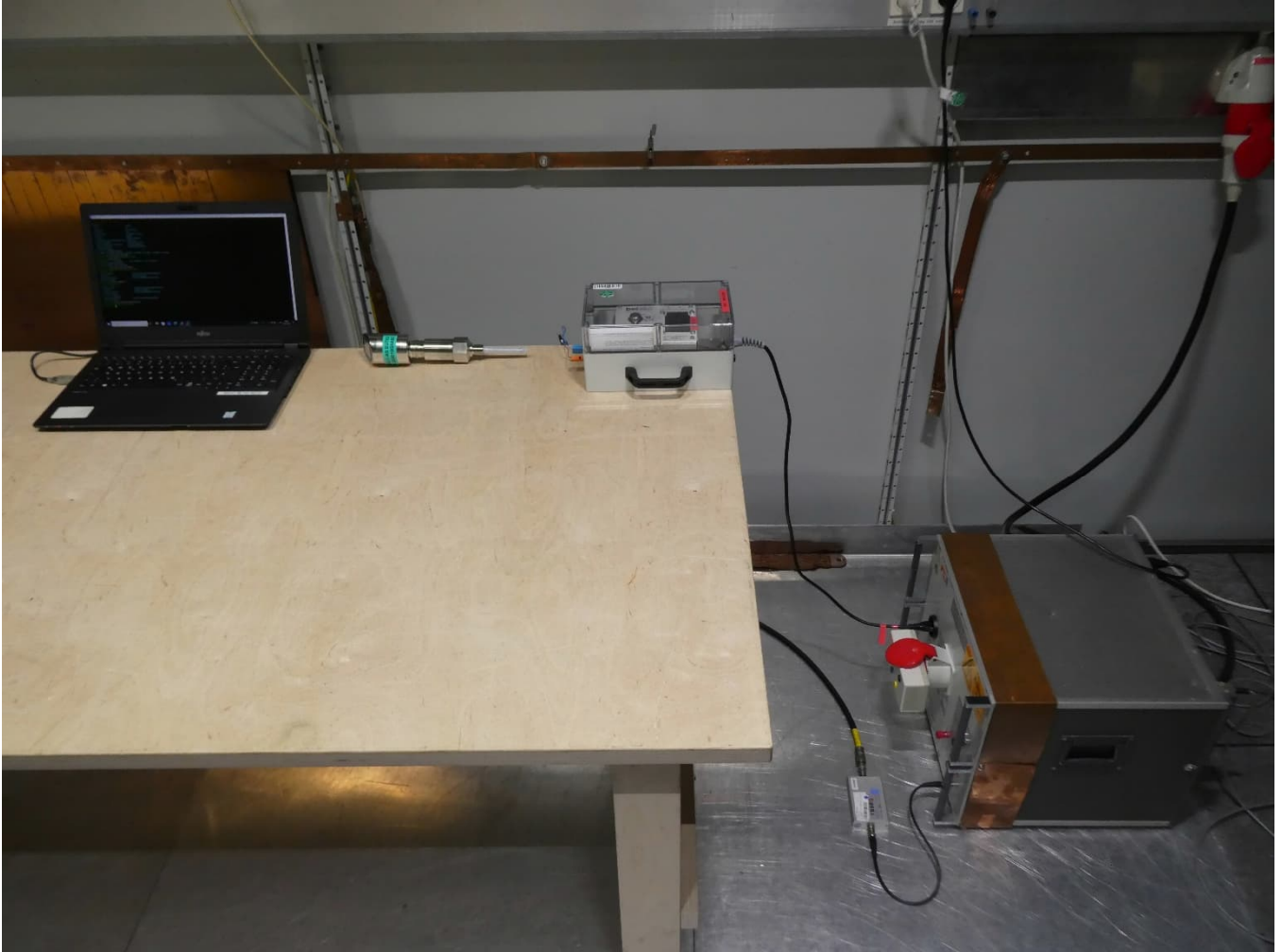
Test setup AC power line conducted emissions - view 1
