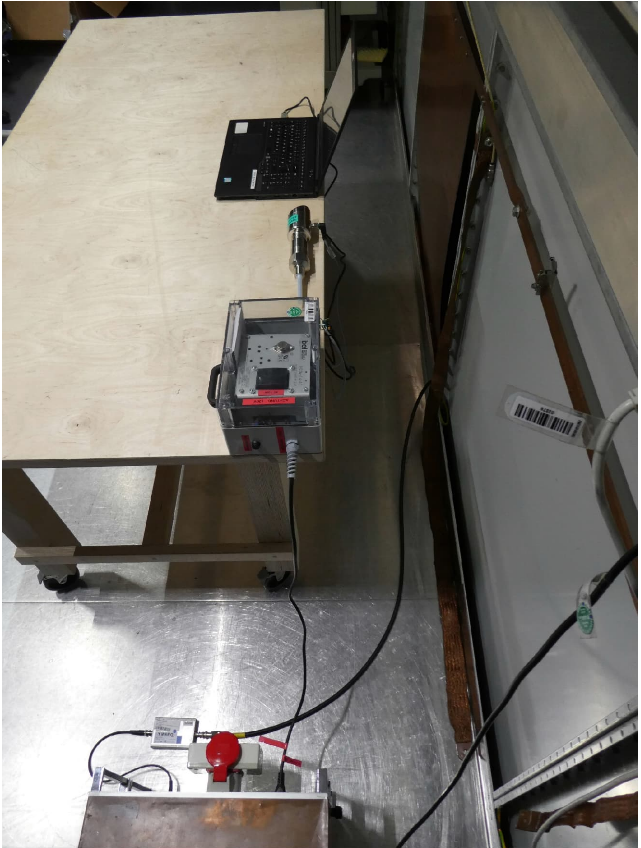
Test setup AC power line conducted emissions - view 2
