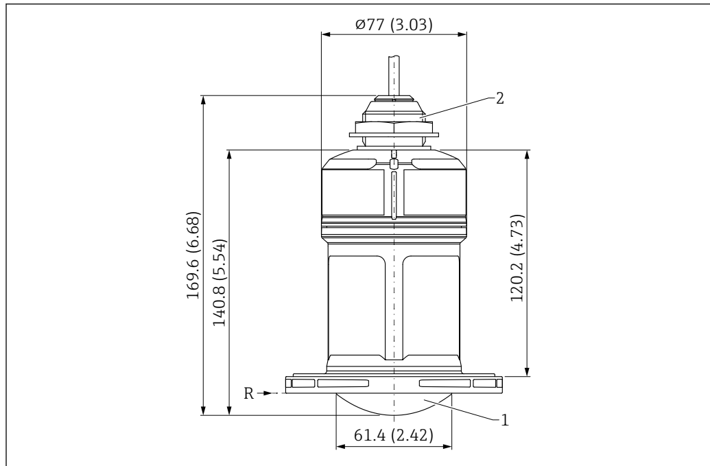
23 Dimensions; 80 mm (3 in) antenna with cable entry from above. Unit of measurement mm (in)
