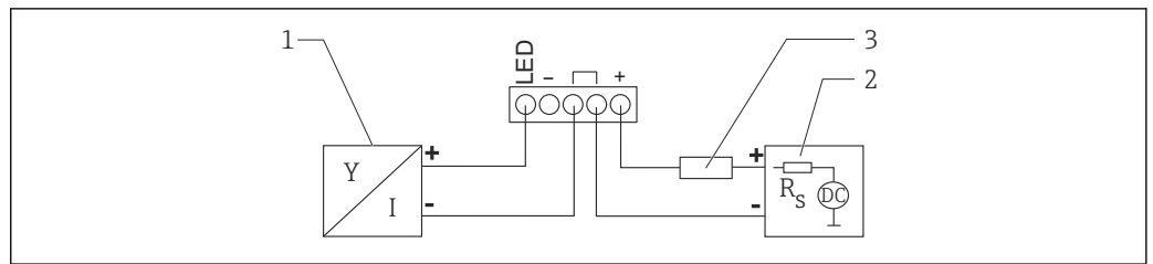
6 Function diagram of HART device with RIA15 process indicator with light
