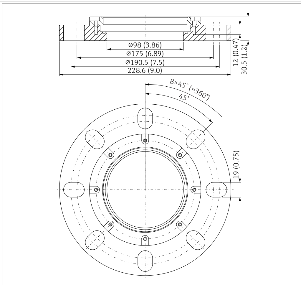
54 Dimensions of UNI slip-on flange 4"/DN100/100. Unit of measurement mm (in)
