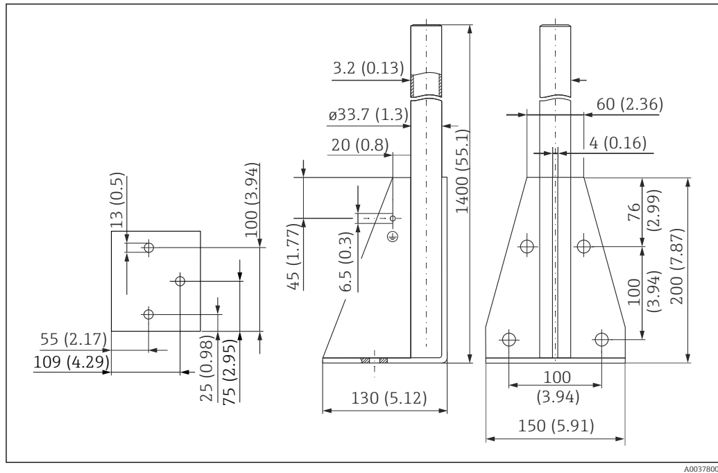
49 Dimensions. Unit of measurement mm (in)
