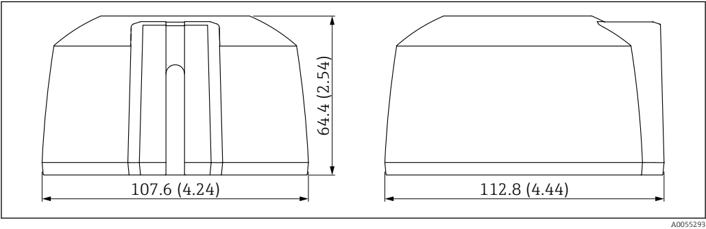
30 Dimensions for protective cover with cable entry at the side. Unit of measurement mm (in)
