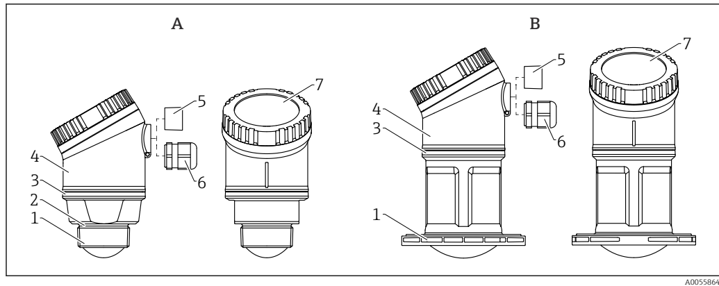
22 Device design
