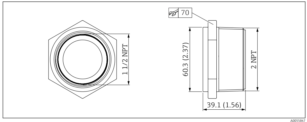
28 Dimensions of Uni adapter
