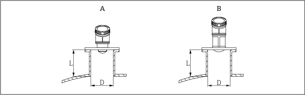
12 Nozzle installation
