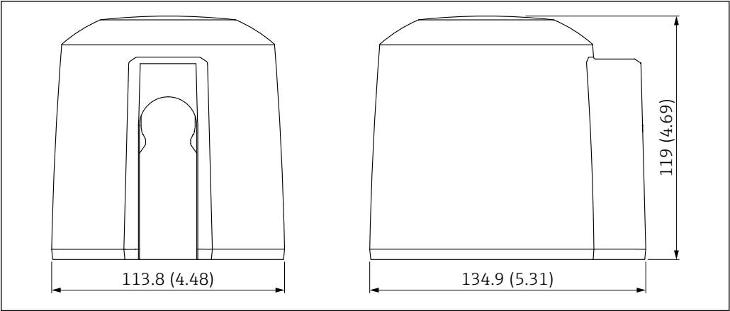
24 Dimensions for weather protective cover . Unit of measurement mm (in)
