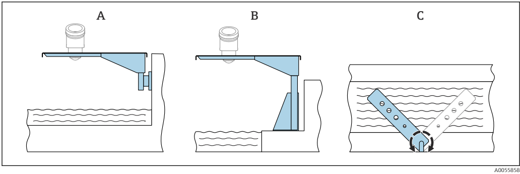
16 Cantilever installation, with pivot A Cantilever with wall bracket (side view) B Cantilever with mounting frame (side view) C Cantilever can be turned, e.g. in order to position the device over the center of the flume (top view)
