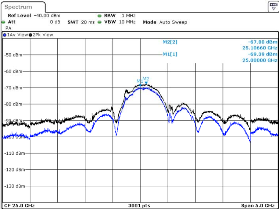
Fundamental Emission - 1MHz RBW, Average, Peak – P5LPR
