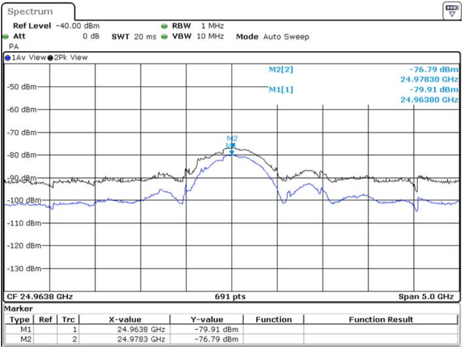
Fundamental Emission - 1MHz RBW, Average, Peak – P2LPR
