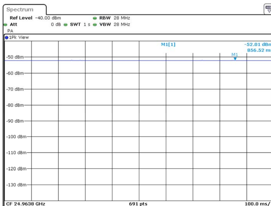
Fundamental Emission - 28 MHz RBW, Peak, Zero Span - P2LPR
