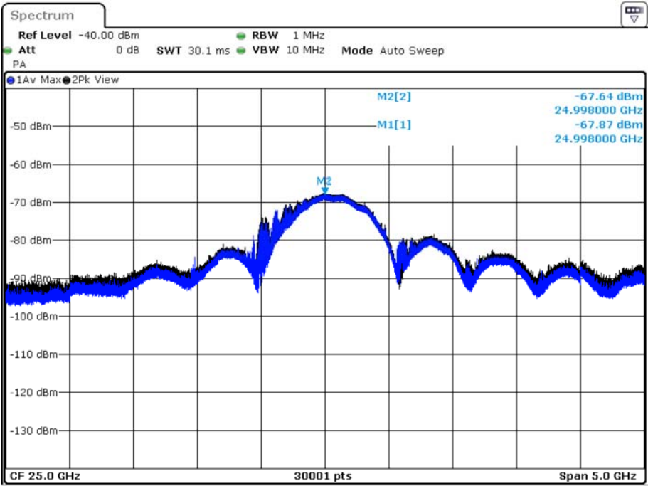
Fundamental Emission - 1MHz RBW, Average, Peak – P4LPR
