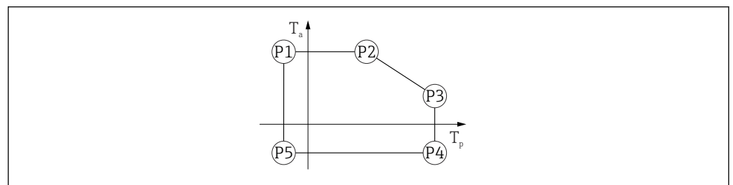
17 Plastic housing material; process temperature range: -20 to +150 °C (-4 to +302 °F)
