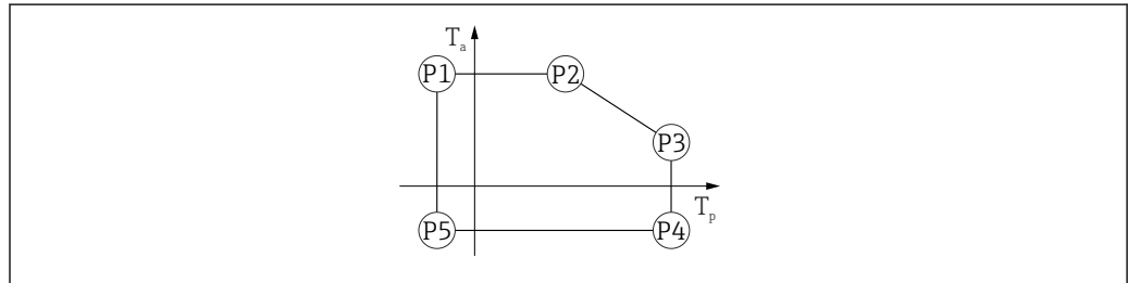
19 Plastic housing material; process temperature range: -20 to +200 °C (-4 to +392 °F)
