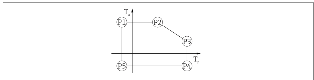
35 316L housing material; process temperature range: -20 to +150 °C ( -4 to +302 °F)
