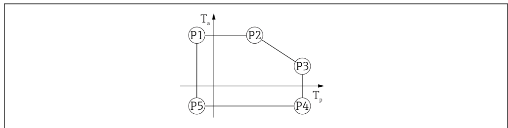
29 Aluminum housing material; process temperature range: -20 to +150 °C ( -4 to +302 °F)
