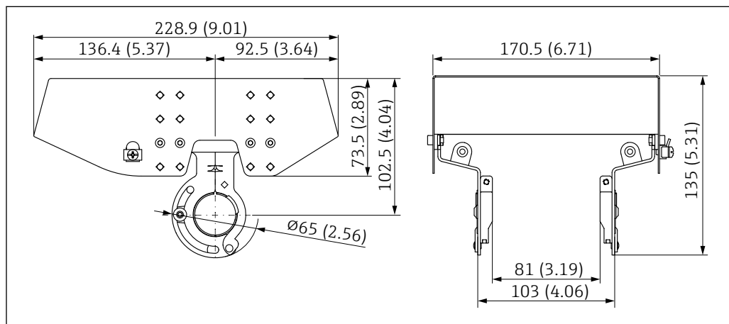
13 Dimensions. Unit of measurement mm (in)
