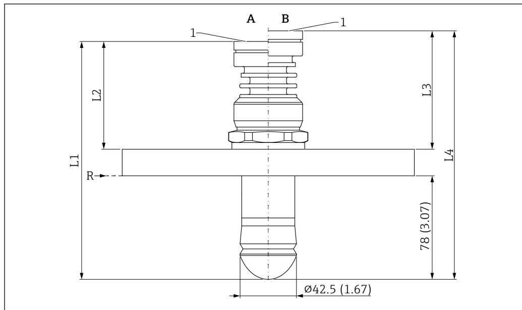
25 Dimensions of Drip-off antenna 50 mm (2 in), UNI flange process connection. Unit of measurement mm (in)
