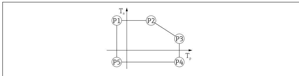
8 Plastic housing material; process temperature range: -40 to +80 °C (-40 to +176 °F)
