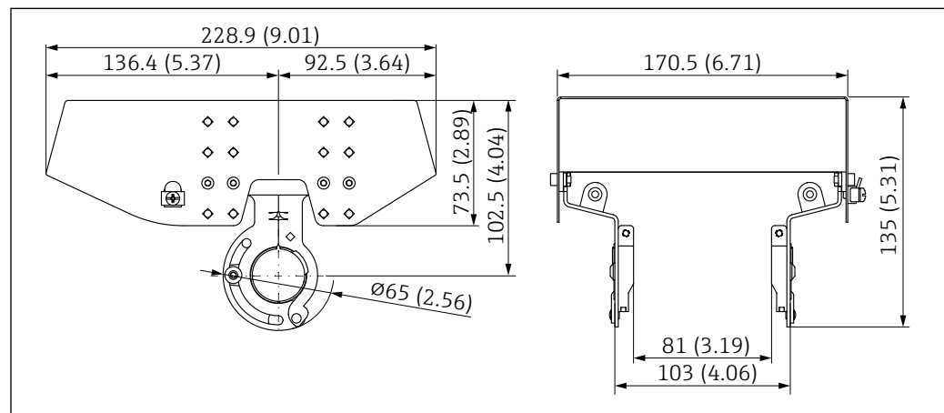
33 Dimensions. Unit of measurement mm (in)
