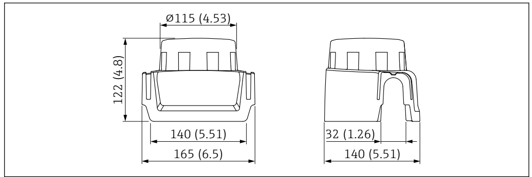
34 Dimensions. Unit of measurement mm (in)
