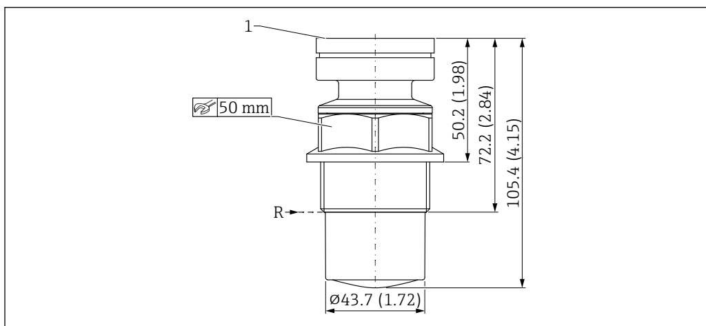
19 Dimensions of encapsulated antenna, PVDF, 40 mm (1.5 in). Unit of measurement mm (in)
