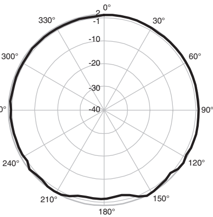
horizontal 2.5 GHz
