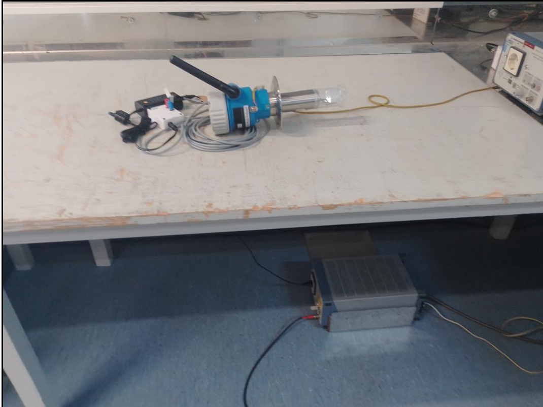
Photo 1: conducted emission
