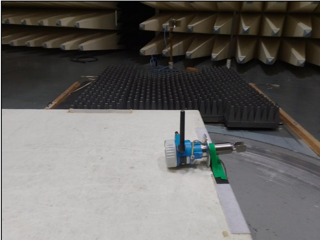
Photo 3: radiated emission >1 GHz
