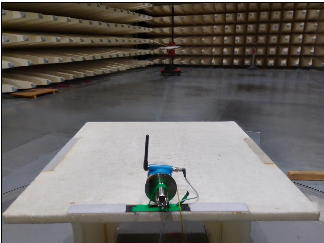
Photo 2: radiated emission <1 GHz
