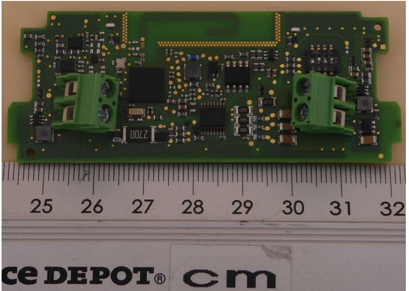
EUT – Main PCB top view
