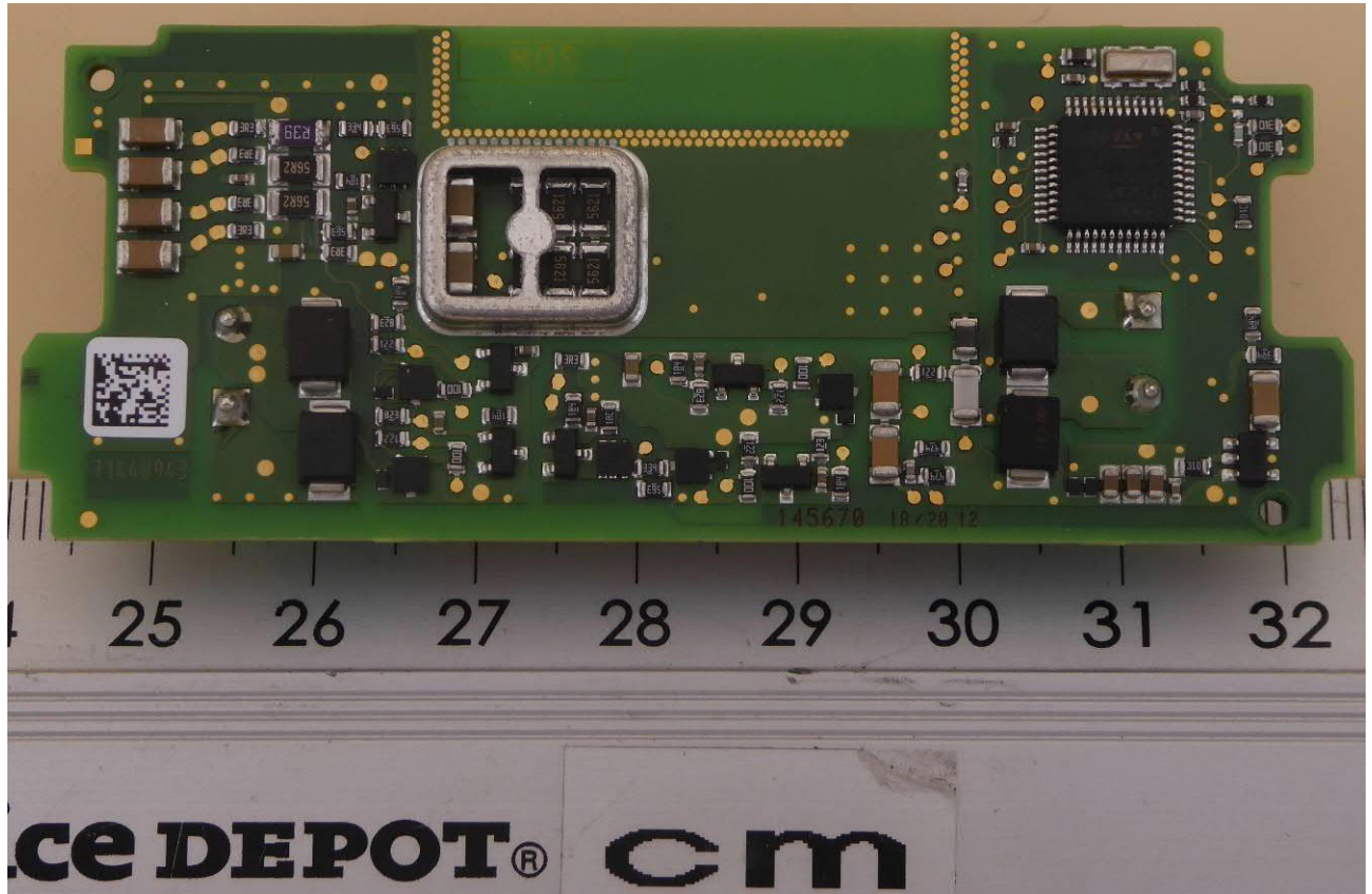
EUT – Main PCB bottom view
