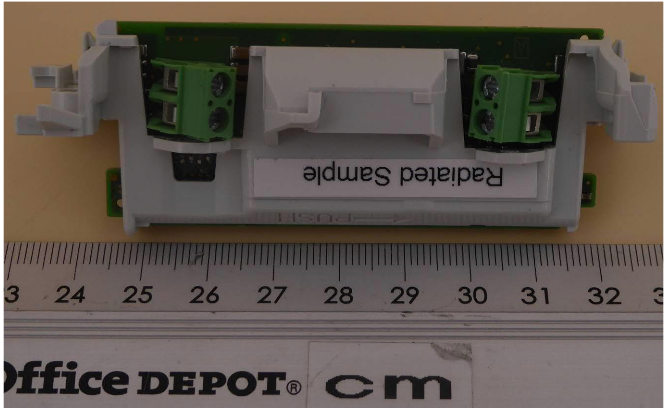
EUT – Main PCB + Housing 1
