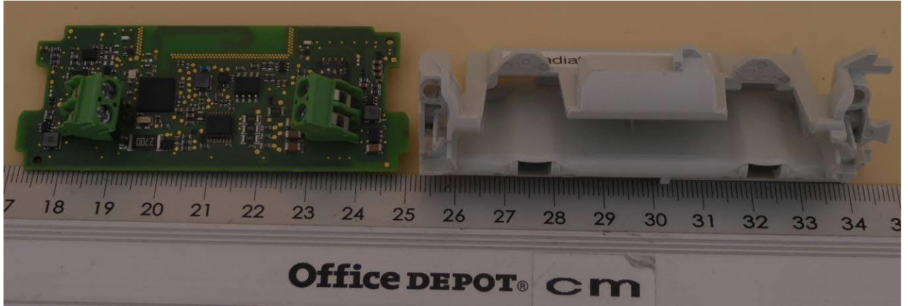
EUT – Main PCB + Housing 2
