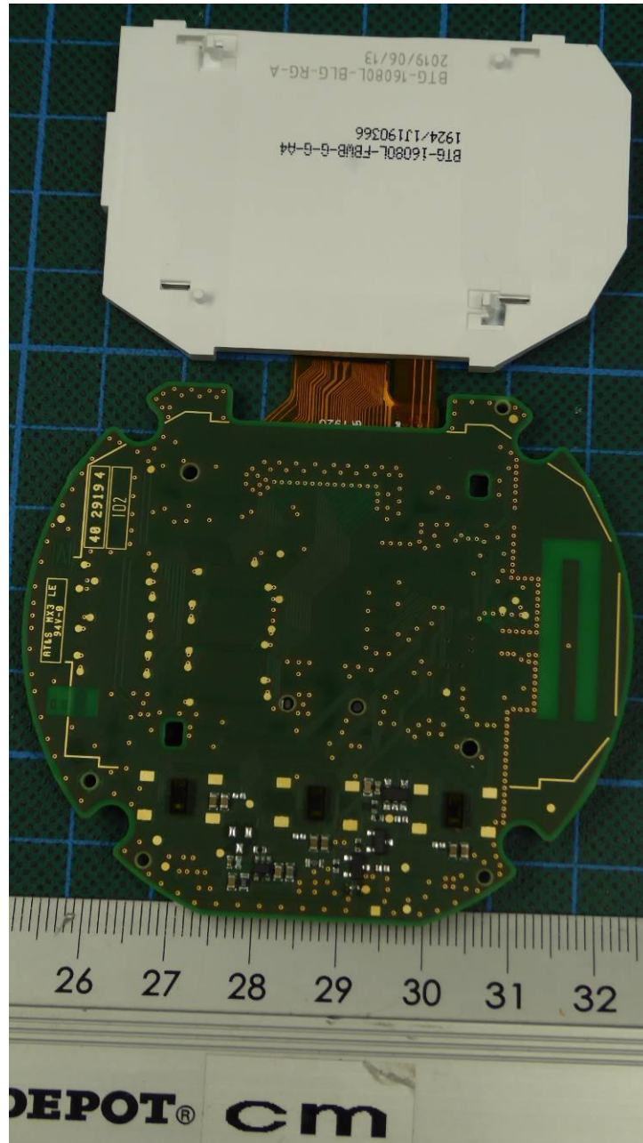
EUT VE113_A_03 – PCP top view (display folded down)
