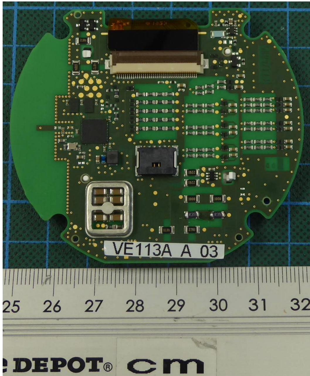
EUT VE113_A_03 – PCP bottom view
