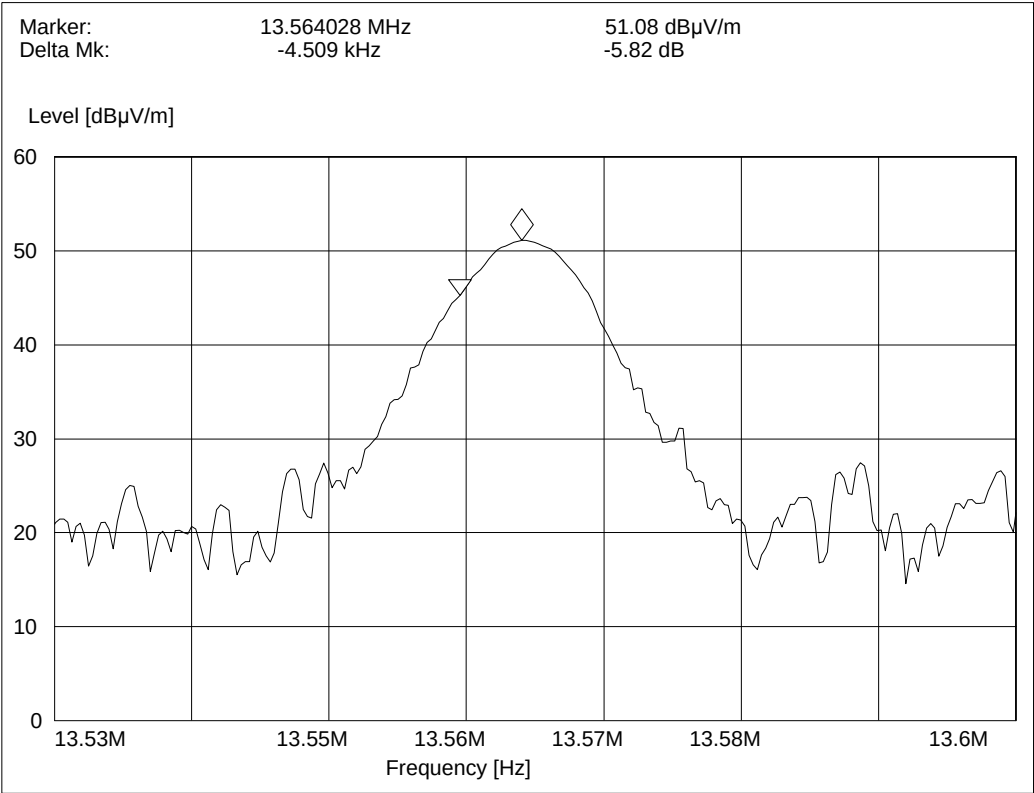
Figure 5 - 13.56MHz Bandwidth Resolution BW:9KHz, VideoBW:30Khz
