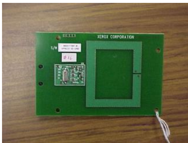
Figure 4 PWBA Detail
