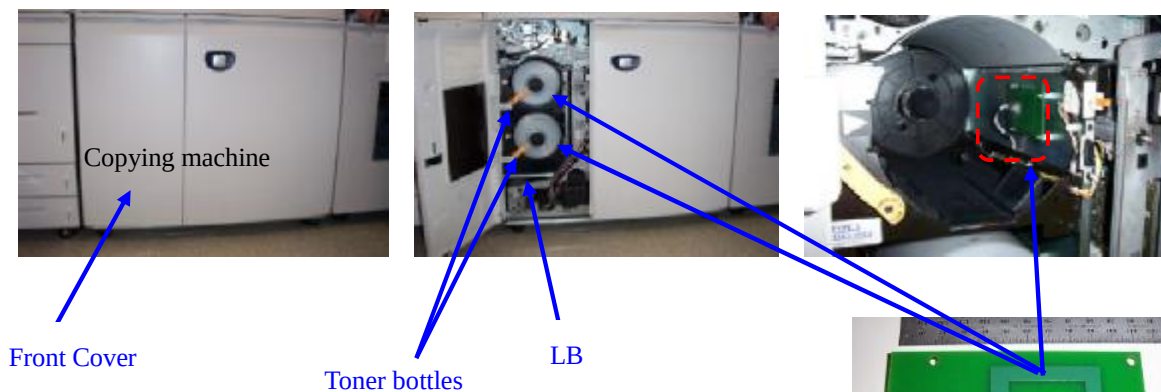
Fig.A-1: Attached position of RRFCS -C to machine
